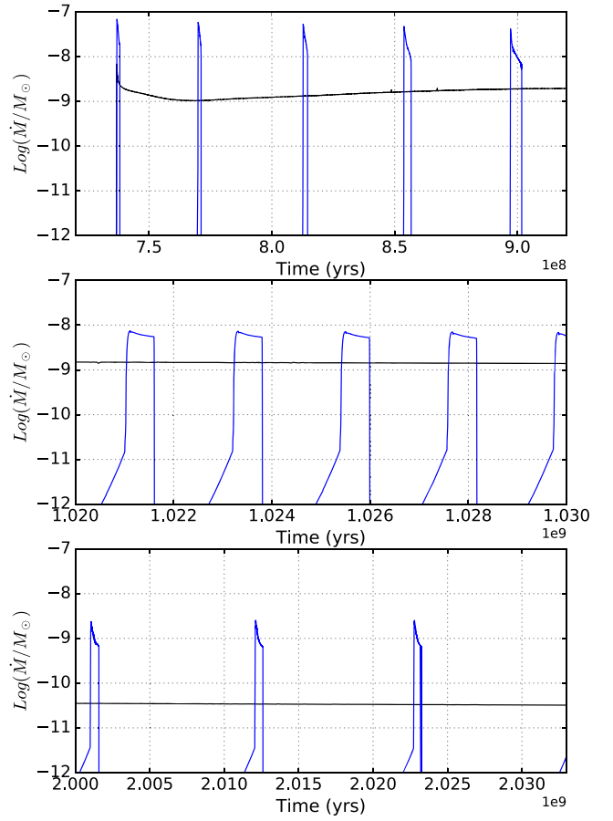
Figure 6. The evolution of the mass lost by the companion (as \text{Log}(M_2/M_\odot) ) during the evolution segments reported in Panels A, B and C of Fig. 1, respectively, in the upper, middle and bottom panels. Each panel highlights the cyclic nature of the irradiated evolution throughout its entire duration.
