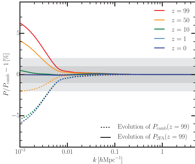
Figure 5. We compare the evolution of two different initial linear power spectra at z = 99 : one is directly taken from CAMB, the other one is obtained with our method, i.e. the z = 0 power spectrum from CAMB has been rescaled to the initial redshift with our two-fluid approximation. The two spectra are then evolved forward using the two-fluid approximation, thus mimicking the linear (Newtonian) evolution in a simulation. In the first case, dashed lines, by construction at high redshift the evolved power spectrum coincides with that from the Boltzmann code, but differs from it at low redshift (reaching a lack of power > 5 percent at large scales at z = 0 ). On the other hand, our rescaling (solid lines) introduces a discrepancy at high redshift and large scales (due to the fact that in our Newtonian approximation all photon perturbations are inevitably neglected), but allows us to recover a sub-percent agreement with the linear power spectrum from a Boltzmann code at lower redshifts ( z < 10 ).
