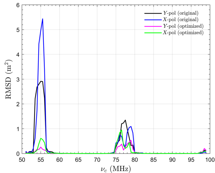
Fig. 10 Local residuals between second-order polynomial models and simulated effective areas shown in Fig. 9 considering narrow-band fittings (2 MHz).
