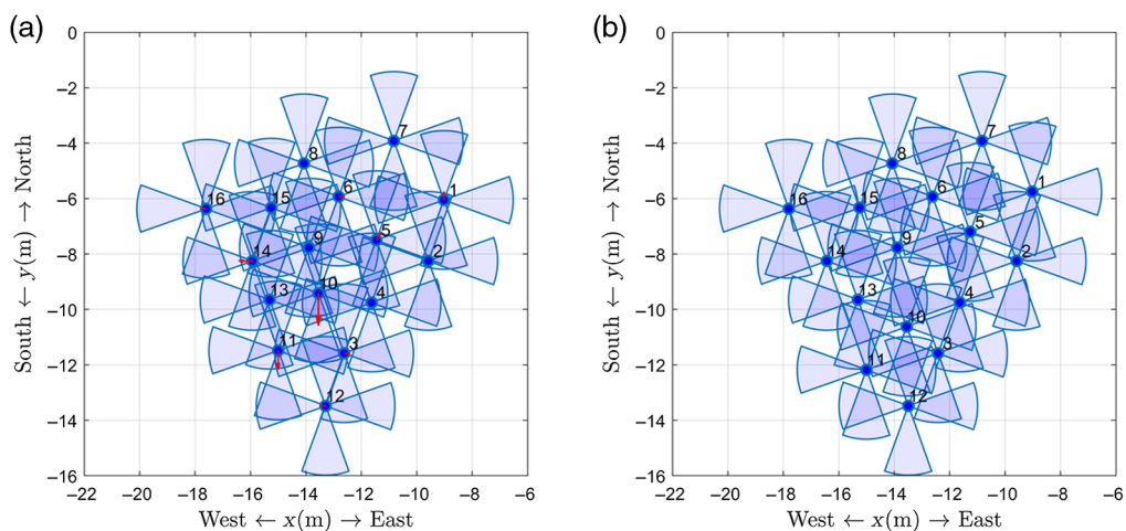
Fig. 7 Antenna distribution for the tile analyzed in this paper: (a) original layout as proposed in AAVS2 and (b) optimized layout considering exclusion zones. The exclusion zones (transparent blue areas) are given by the sector of circumferences of 2.5 m radius and \pm 20 deg with respect to the main axis. The arrows in (a) shows the translations applied to the antennas to obtain the layout of (b).
