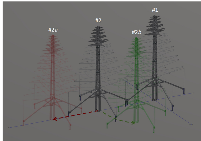
Fig. 1 Geometry of the model with two SKALA4.1 antennas. The antenna in the origin (#1) is fixed, whereas the position of the second antenna (#2) varies either along the X axis (up to 2.7 m, #2a) or along a circular trajectory centered in the origin with a radius of 1.5 m (up to 45 deg, #2b). The colored arrows and the transparent SKALA4.1 antennas describe the different extremes of the two movements of the second antenna.
