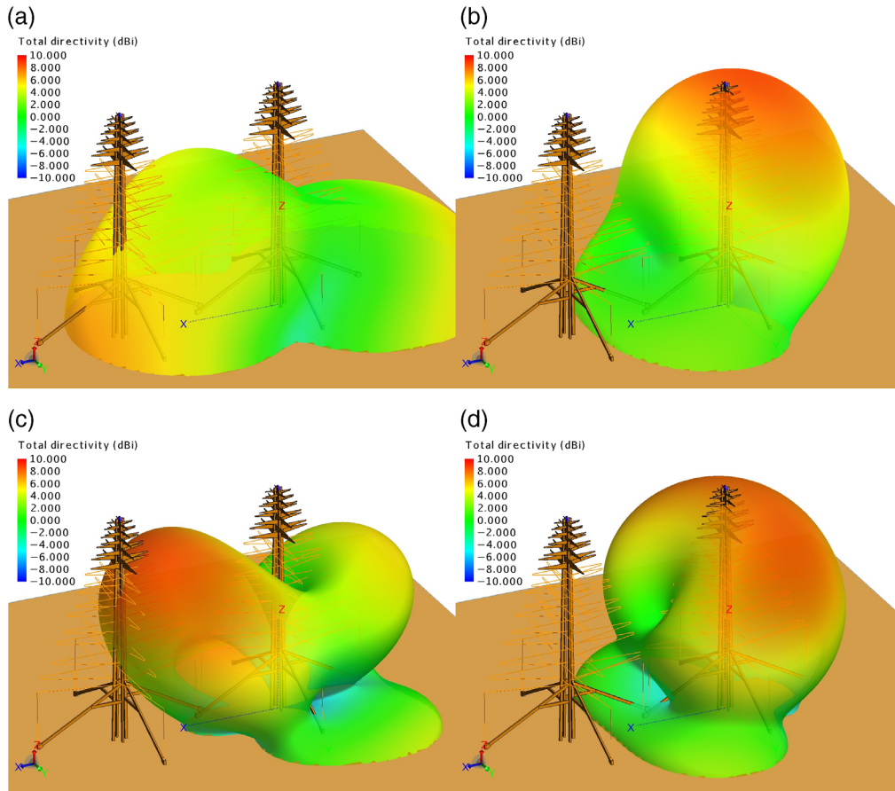
Fig. 5 3D antenna patterns for the X-polarized SKALA4.1 #1 antenna (on the right side of each subplot) in the presence of the SKALA4.1 #2 (on the left side). Four different frequencies were considered: (a) 54.5 MHz, (b) 57 MHz, (c) 77 MHz, and (d) 78 MHz.
