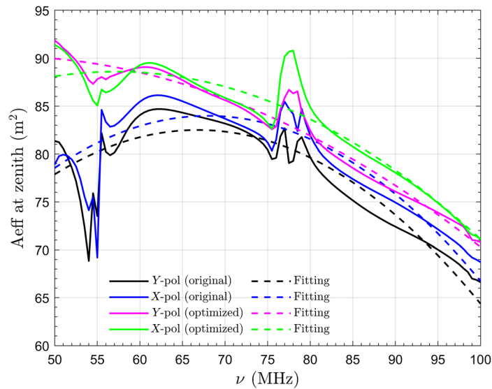
Fig. 9 Effective area at zenith (continuous curves) between 50 and 100 MHz for both polarizations of a tile of 16 SKALA4.1 antennas. Blue and black curves refer to the nominal layout, whereas green and magenta curves are the optimized layout. Dashed curves represent the second-order polynomial fitting.
