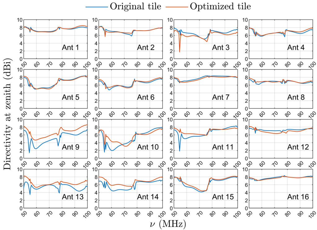
Fig. 8 Directivity at zenith in the frequency band 50 to 100 MHz for each antenna composing one tile of AAVS2. The original tile layout is the blue curves; the optimized tile layout is the orange curves.
