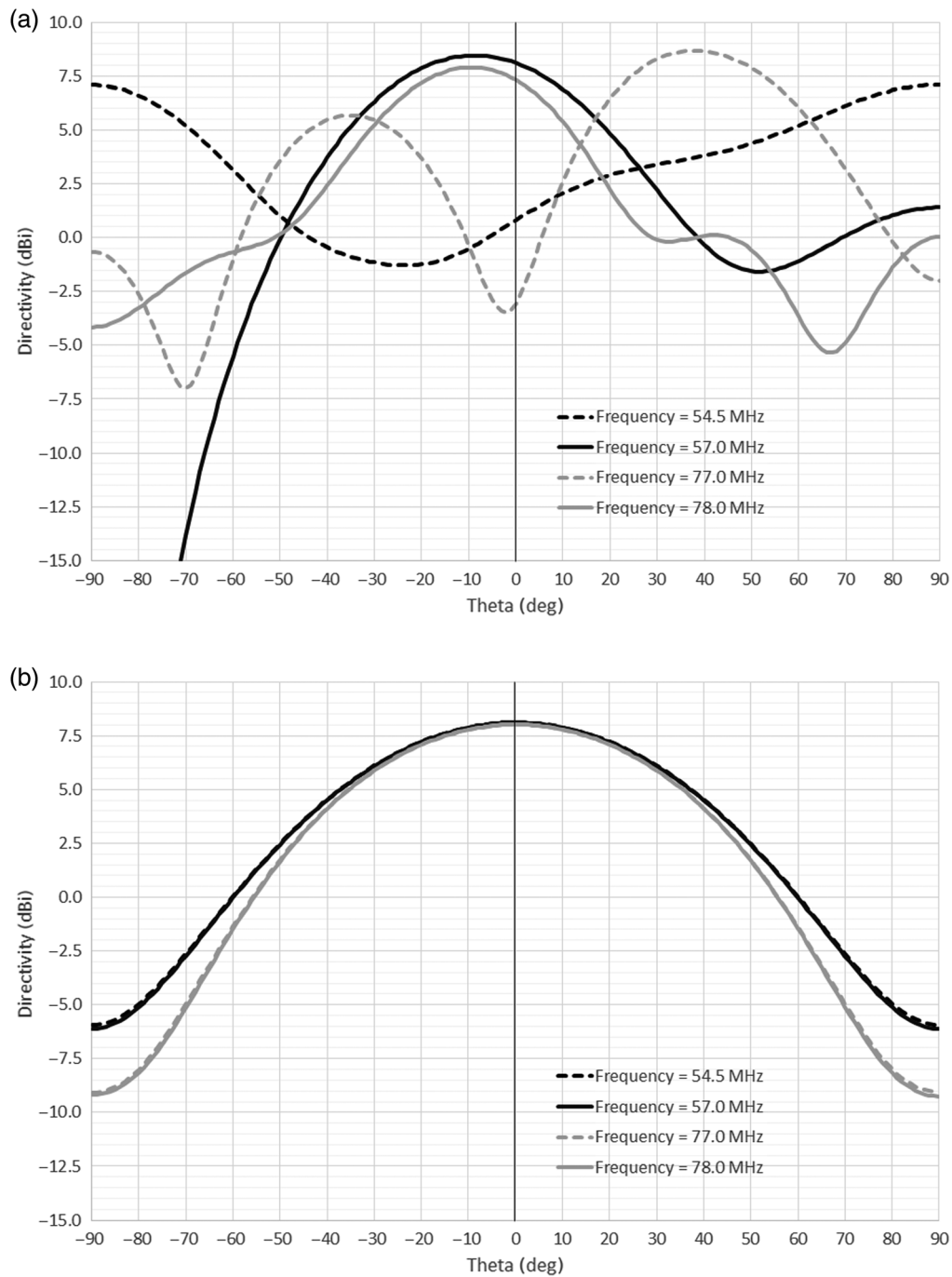
Fig. 4 Antenna patterns in the E plane for the X-polarized SKALA4.1 #1 antenna for two different scenarios: (a) in the presence of the SKALA4.1 #2 located at X = 1.5 m and Y = 0 m and (b) isolated. The patterns are shown at four different frequencies: 54.5 and 77 MHz corresponding to the minimum directivity at zenith and at 57 and 78 MHz used as reference.
