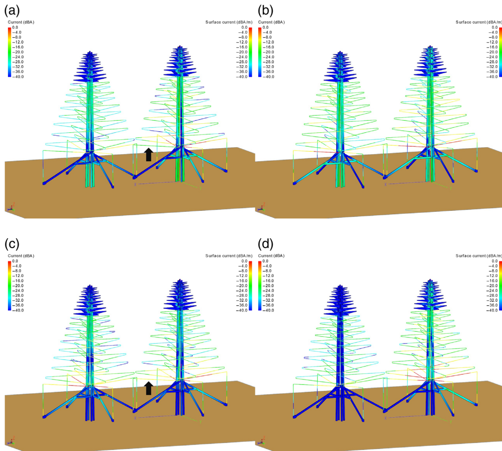
Fig. 6 Normalized linear and surface current distributions with the X-polarized SKALA4.1 #1 (right antenna) excited at four frequencies: (a) 54.5 MHz, (b) 57 MHz, (c) 77 MHz, and (d) 78 MHz. The black arrows in (a) and (c) identify, in the active antenna, the half of the bottom bow-tie dipole weakly excited at the resonant frequencies.
