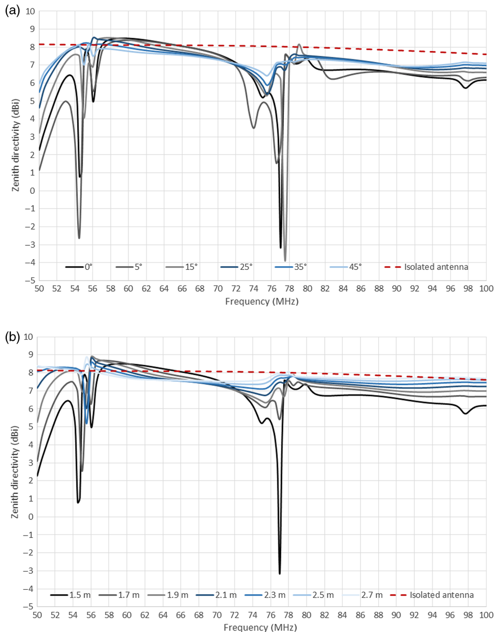
Fig. 2 Directivity at zenith in the frequency band 50 to 100 MHz for the X-polarized SKALA4.1 #1 antenna centered in the origin. The continuous curves correspond to a different position of the second antenna (SKALA4.1 #2) as described in Fig. 1, whereas the dashed red curve is the isolated antenna response. (a) The case of circular trajectory and (b) the linear shift.
