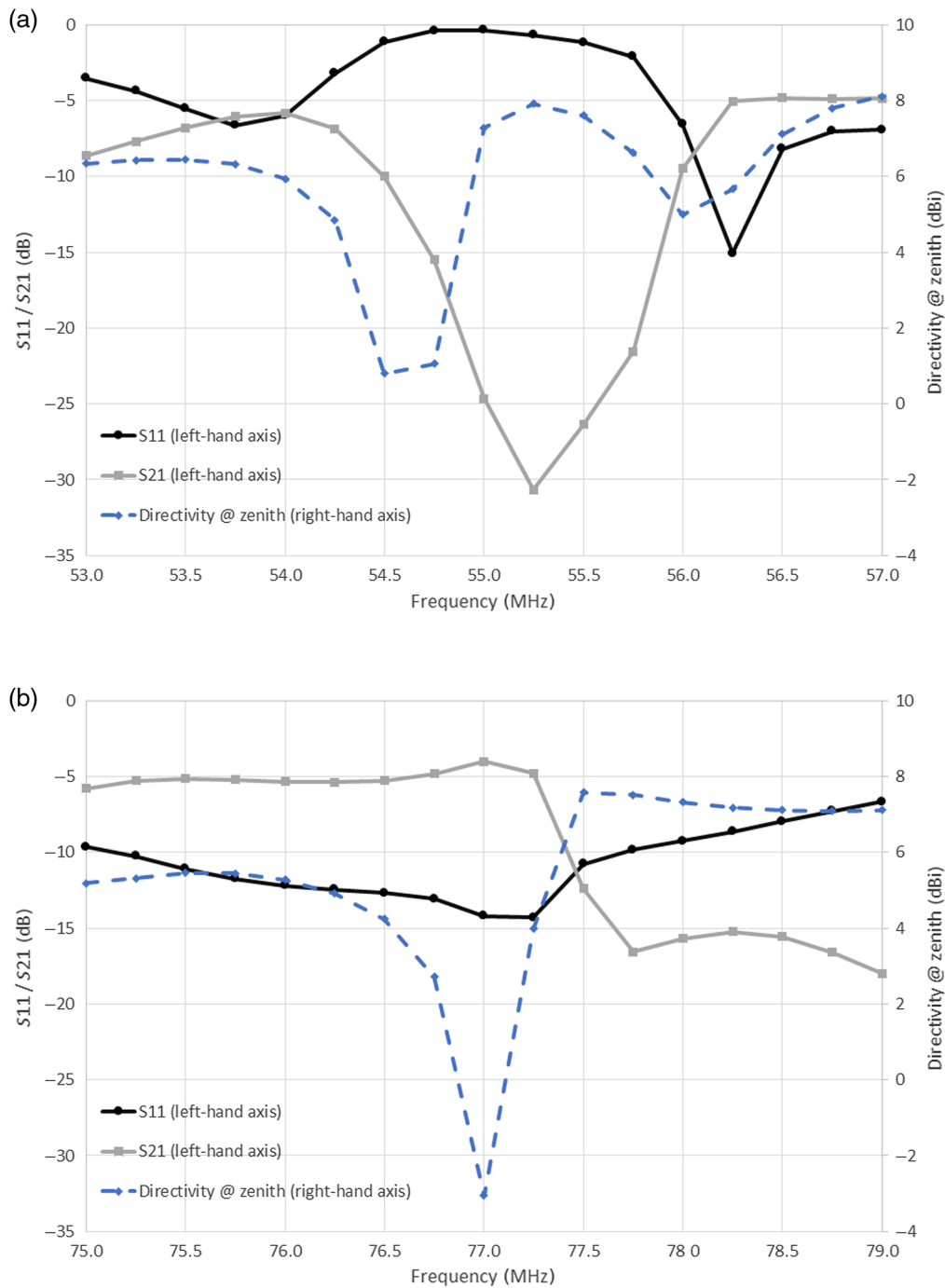
Fig. 3 Directivity at zenith, reflection coefficient, and mutual coupling coefficient for the X-polarized SKALA4.1 #1 antenna with a second antenna SKALA4.1 #2 located at X = 1.5 m and Y = 0 m. (a) The frequency bands 53 to 57 MHz and (b) 75 to 79 MHz.
