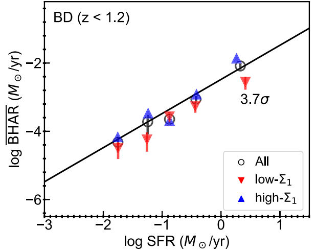
Figure E1. \overline{\text{BHAR}} versus SFR for BD galaxies with \log M_* > 10 at z < 1.2 in the COSMOS field divided into SFR bins with \approx 1000 sources per bin. Each SFR bin (black circles) is further divided into two subsamples with \Sigma_1 above (blue upward-pointing triangles) and below (red downward-pointing triangles) the median \Sigma_1 of the bin, respectively. The black solid line represents the best-fitting \overline{\text{BHAR}}-\text{SFR} relation in Yang et al. (2019). We can see that the general \overline{\text{BHAR}}-\text{SFR} trend is close to that obtained in Yang et al. (2019).
