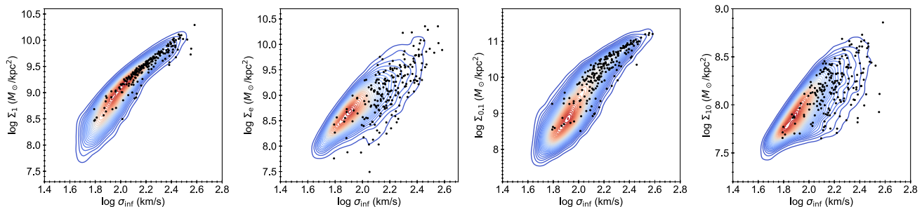
Figure 10. Left to right: 2D kernel density estimation (KDE) plot of \Sigma_1 , \Sigma_e , \Sigma_{0.1} , and \Sigma_{10} versus \sigma_{\text{inf}} of galaxies in the ALL SF sample. X-ray detected galaxies are represented by the black dots. Note the correlation between \sigma_{\text{inf}} and \Sigma_1 is tighter than the correlations between \sigma_{\text{inf}} and other compactness parameters shown.
