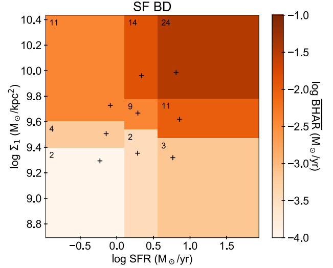
Figure 5. Colour-coded \overline{\text{BHAR}} in different bins of SFR and \Sigma_1 for galaxies in the SF BD sample. Each 2D bin contains \approx 110 sources. The black plus sign indicates the median SFR and \Sigma_1 of the sources in each bin. For each bin, the number of X-ray detected galaxies is listed.
