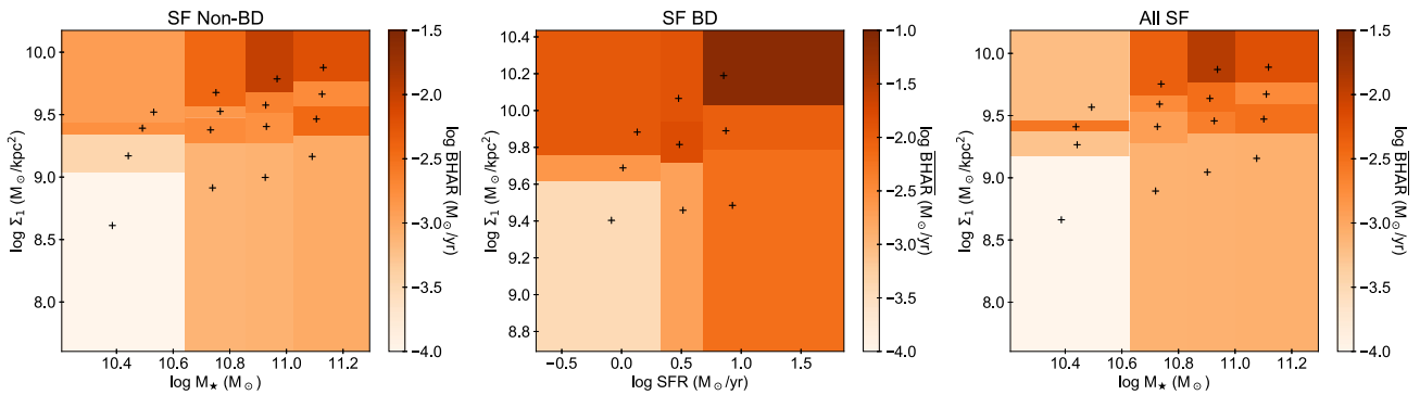
Figure D1. Left-hand panel: colour-coded \overline{\text{BHAR}} in different bins of M_* and \Sigma_1 for galaxies in the SF non-BD sample. Each 2D bin contains \approx 11 X-ray detected galaxies. The black plus sign indicates the median M_* and \Sigma_1 of the sources in each bin. Middle panel: colour-coded \overline{\text{BHAR}} in different bins of SFR and \Sigma_1 for galaxies in the SF BD sample. Each 2D bin contains \approx 9 X-ray detected galaxies. The black plus sign indicates the median SFR and \Sigma_1 of the sources in each bin. Right-hand panel: colour-coded \overline{\text{BHAR}} in different bins of M_* and \Sigma_1 for galaxies in the ALL SF sample. Each 2D bin contains \approx 13 X-ray detected galaxies. The black plus sign indicates the median M_* and \Sigma_1 of the sources in each bin.
