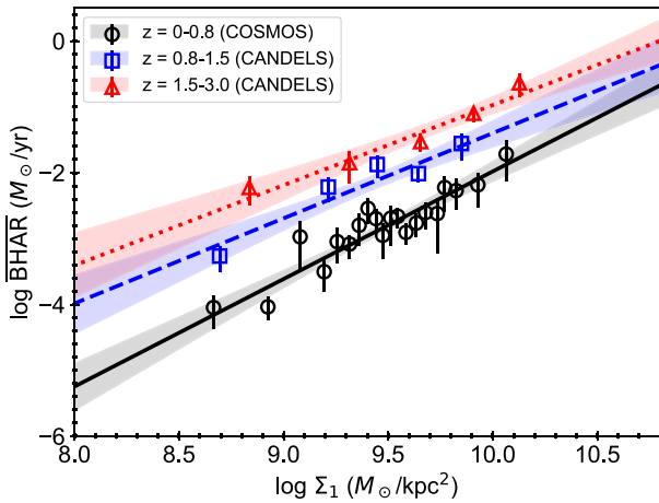
Figure 8. The cosmic evolution of the \overline{\text{BHAR}}-\Sigma_1 relation among SF galaxies. z = 0-0.8 galaxies from COSMOS, z = 0.8-1.5 galaxies from CANDELS, and z = 1.5-3 galaxies from CANDELS with \log M_* > 10.2 are divided into several bins according to their \Sigma_1 values with approximately the same number of X-ray detected galaxies in each bin, represented by the black circles, blue squares, and red triangles, respectively. The horizontal position of each data point indicates the median \Sigma_1 of the sources in the bin; the error bars represent the 1\sigma confidence interval of \overline{\text{BHAR}} from bootstrapping. The black solid line and the grey shaded region represent the best-fitting \overline{\text{BHAR}}-\Sigma_1 relation and its 1\sigma/3\sigma pointwise confidence interval for z = 0-0.8 galaxies; the blue dashed line and the blue shaded region are for the z = 0.8-1.5 galaxies; and the red dotted line and the red shaded region are for the z = 1.5-3 galaxies.
