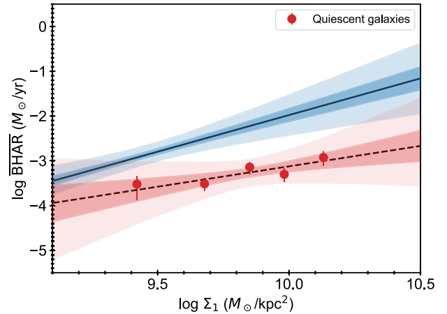
Figure 9. The \overline{\text{BHAR}}-\Sigma_1 relation among quiescent galaxies. 3400 quiescent galaxies with \log M_* > 10.2 at z < 0.8 are divided into bins according to their \Sigma_1 values, with \approx 20 X-ray detected galaxies in each bin. The horizontal position of each data point indicates the median \Sigma_1 of the sources in the bin; the error bars represent the 1\sigma confidence interval of \overline{\text{BHAR}} from bootstrapping. The black dashed line and the dark/light red shaded region represent the best-fitting \overline{\text{BHAR}}-\Sigma_1 relation among quiescent galaxies and the 1\sigma/3\sigma pointwise confidence intervals on the regression line, respectively. The black solid line and the dark/light blue shaded region are adopted from Fig. 7, representing the best-fitting \overline{\text{BHAR}}-\Sigma_1 relation among SF galaxies in the same M_* and z ranges and the 1\sigma/3\sigma pointwise confidence intervals on the regression line, respectively. At a given \Sigma_1 , the \overline{\text{BHAR}} values of quiescent galaxies are below the 3\sigma lower limit of the best-fitting \overline{\text{BHAR}}-\Sigma_1 relation among SF galaxies, and the best-fitting slope of the \log \overline{\text{BHAR}}-\log \Sigma_1 relation among quiescent galaxies is much flatter compared with the best-fitting slope among SF galaxies.
