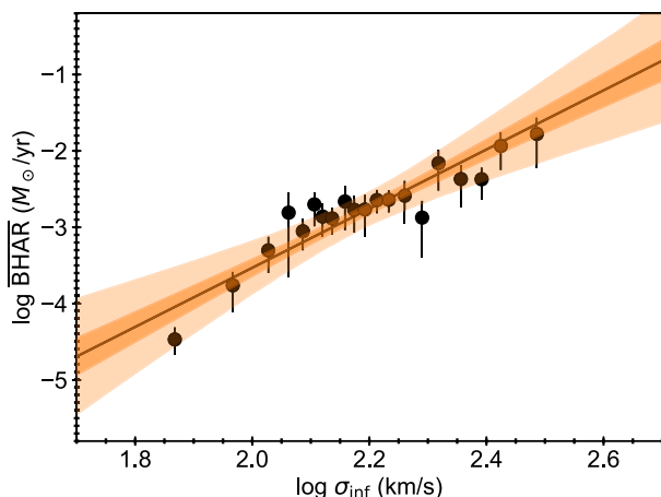
Figure 11. \overline{\text{BHAR}} as a function of \sigma_{\text{inf}} among SF galaxies. Galaxies in the ALL SF sample are divided into bins according to their \sigma_{\text{inf}} values, with \approx 10 X-ray detected galaxies in each bin. The horizontal position of each data point indicates the median \sigma_{\text{inf}} of the sources in the bin; the error bars represent the 1\sigma confidence interval of \overline{\text{BHAR}} from bootstrapping. The black solid line and the dark/light orange shaded region represent the best-fitting \overline{\text{BHAR}}-\sigma_{\text{inf}} relation and the 1\sigma/3\sigma pointwise confidence intervals on the regression line, respectively.
