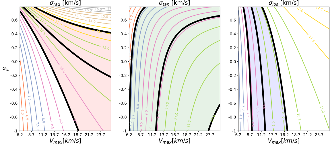
Fig. 13. Velocity dispersion maps in the V_{\max} -anisotropy space. Left, central and right panels show the velocity dispersions in the projected radial, tangential and in the LOS components, respectively. Black solid lines and coloured-shaded areas indicate the range defined by our mean measurements and their 16th and 84th percentiles, at R_{HST} . Coloured lines indicate contours of constant dispersion in steps of 0.5 km/s.
