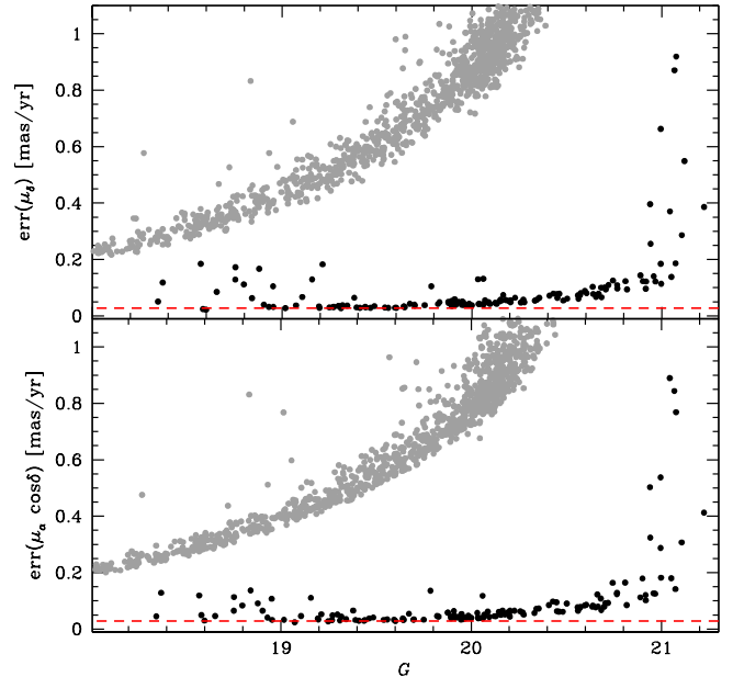
Fig. 4. Intrinsic uncertainties as a function of Gaia G -band magnitude for the proper-motion component along \alpha (lower panel) and \delta (upper panel). Black-filled symbols are our HST+ Gaia estimates, while grey-filled symbols are Gaia DR2 proper-motion uncertainties for sources in the direction of Draco. The red dashed line corresponds to a velocity of 10 km/s at the distance of Draco, roughly mimicking the system velocity dispersion.
