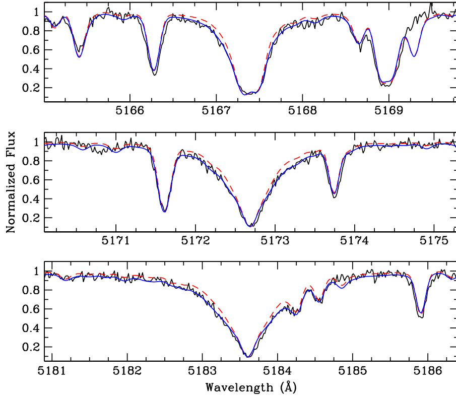
Figure 4. Comparison between the observed spectrum (solid black line) and two synthetic spectra for the Mg I lines at 5167.3, 5172.6 and 5183.6 \text{\AA} . The synthetic spectra have been computed by adopting T_{\text{eff}} = 5013 \text{ K} and v_{\text{turb}} = 1.20 \text{ km s}^{-1} and by adopting two different values of the surface gravity: \log g = 2.03 \text{ dex} corresponding to a stellar mass of 0.6 M_{\odot} (dashed red line) and \log g = 2.40 \text{ dex} corresponding to 1.4 M_{\odot} (solid blue line). Clearly, the spectrum obtained for a 0.6 M_{\odot} star is unable to reproduce the observations, while the observed wings of the Mg I b triplet are very well matched under the assumption of a 1.4 M_{\odot} stellar mass.
