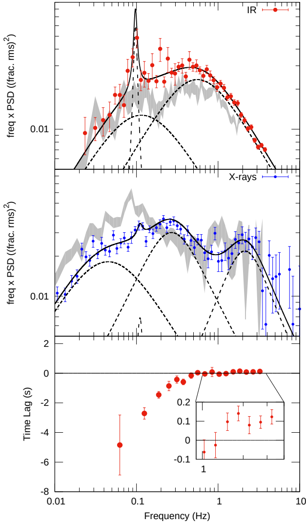
Figure 2. Results from the Fourier analysis of the strictly simultaneous observation on the 17th of September 2015. Top panels: PSDs computed with 1024 (IR) and 16384 (X-ray) bins per segments. The dotted lines indicate the Lorentzian components used to model the PSDs. The grey curves represent the PSDs measured on the last epochs of the campaign, namely on the 3rd of October (X-rays) and 30th of September (IR), for comparison. Bottom panel: frequency dependent time-lags, computed with 128 bins per segment. Positive lags imply IR lagging the X-rays. Spectral coherence
