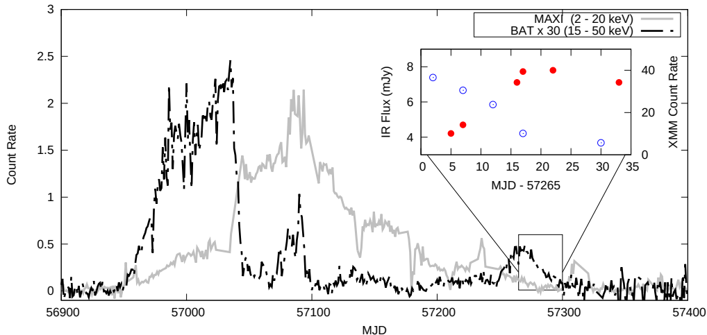
Figure 1. Long term light curve measured by MAXI (grey solid curve) and Swift BAT (black line-dotted curve). The inset shows the evolution of the IR flux (red full points) and the 3-10 keV X-ray count rate measured by XMM (blue empty points) as a function of time during our campaign. The reference date for the light curve in the inset is 31/08/2015.
