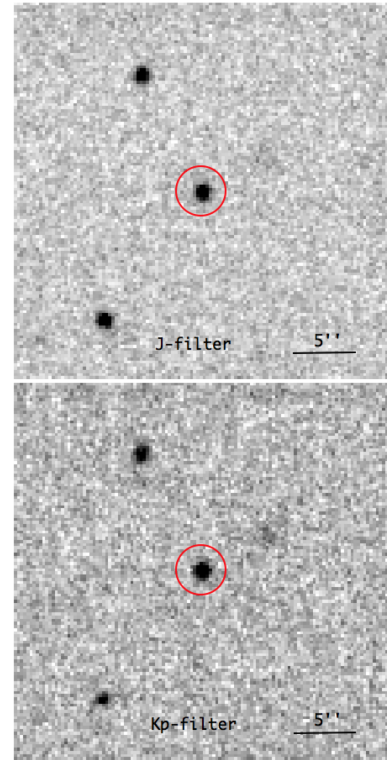
Fig. 2. 0.5' \times 0.5' J and K' cutout images of PSO J0309+27 taken with the LF camera mounted on the NICS instrument. Its optical position is marked with a red circle of 2'' of diameter. The two images are oriented with north up and east to the left.
