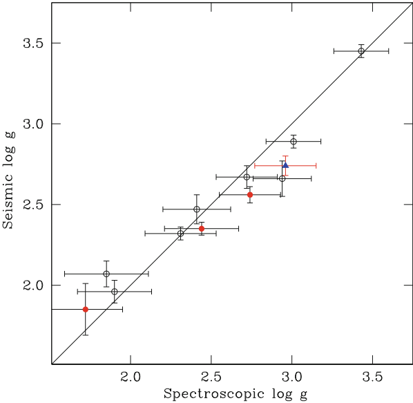
Fig. 2 Agreement between \log g values obtained from seismic and spectroscopic analyses. Red filled circles : red giants belonging to NGC 6633; blue filled triangle : HD 170031; black empty circles : galactic red giants (Color figure online)
