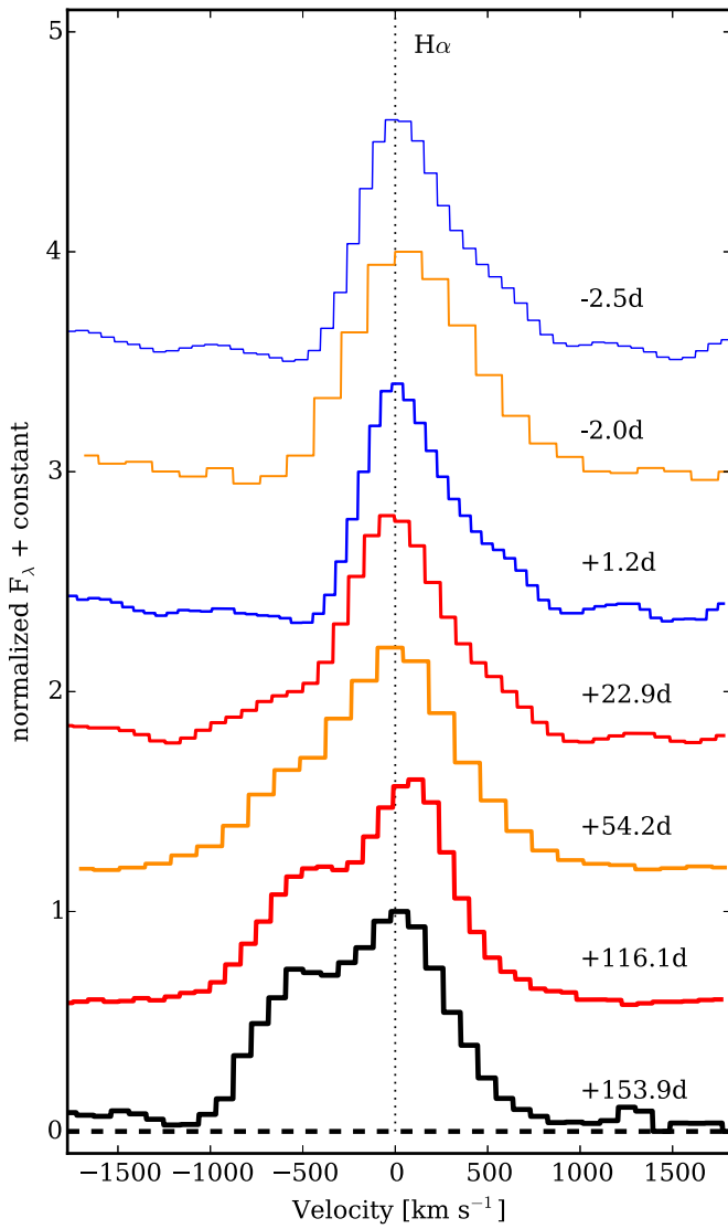
Figure 6. The continuum-subtracted and peak-normalized H \alpha region for DBSP (500 km s ^{-1} ), WHT (320 km s ^{-1} ), NOT (747 km s ^{-1} ) and GTC (380 km s ^{-1} ) spectra. The spectrum is color coded by instrument, the same as in Figure 5.
