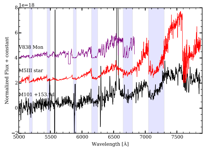
Figure 7. Comparison of M101-OT spectrum at +154 days with HD118767 M5III star (Bagnulo et al. 2003) and the average spectrum of V838 Mon (Tyndea et al. 2011). The spectrum has an estimated blackbody temperature of \sim 3000 K. The molecular bands are comparable to the ones in cool giant stars. Major molecular absorption lines are marked in the spectrum with blue vertical bands.
