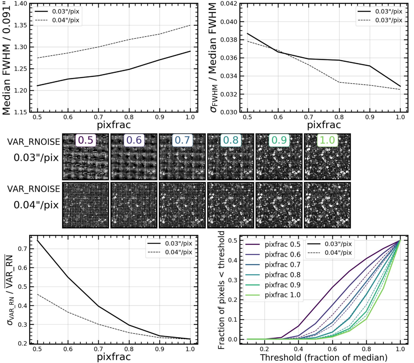
Figure 13. Example of the drizzle tests we performed with simulated images containing 72 point sources and varying the output pixel scales and pixfrac values. The plots here show results for F277W, for which we explored 0''.03 and 0''.04 \text{ pixel}^{-1} output pixel scales. In the top row we show the median recovered FWHM normalized by intrinsic FWHM (left) and the standard deviation of the 72 recovered FWHMs normalized by the median (right), both as a function of pixfrac . In the middle panels, we show small regions of the VAR_RNOISE arrays for each pixel scale and pixfrac , all plotted with the same image stretch and scale. These panels illustrate the decreasing read noise with increasing pixel scale and/or pixfrac . In the bottom left panel we show the normalized image standard deviation of sigma-clipped pixel values in the VAR_RNOISE as a function of pixfrac . In the bottom right panel we plot the fraction of pixels in the inverse VAR_RNOISE arrays that lie below various thresholds as a way to quantify the number of outlier pixels in each mosaic. These tests informed our choice to adopt an output pixel scale of 0''.03 \text{ pixel}^{-1} and a pixfrac of 1 for the mosaics in our first data release.
