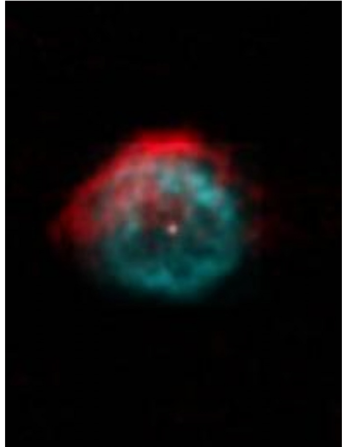
Figure 8. Composite image of IRAS 18576+0341 obtained by superposition of radio images at 6 cm (red) and 17.65 \mu\text{m} (blue).
