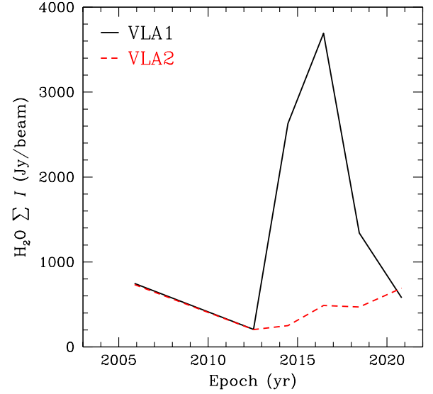
Fig. 6. Comparison of the total sum of the H 2 O maser intensity ( I ) measured toward VLA1 and VLA2 with the VLBI in epochs 2005.89 (VLBA, S11a), 2012.54 (VLBA, S14), 2014.46 (EVN), 2016.45 (EVN), 2018.44 (EVN), and 2020.82 (EVN). The lowest intensities coincide with the minimum of activity registered toward W75N(B) by the 22-m Pushchino telescope in May–July 2012 (Krasnov et al. 2015).
