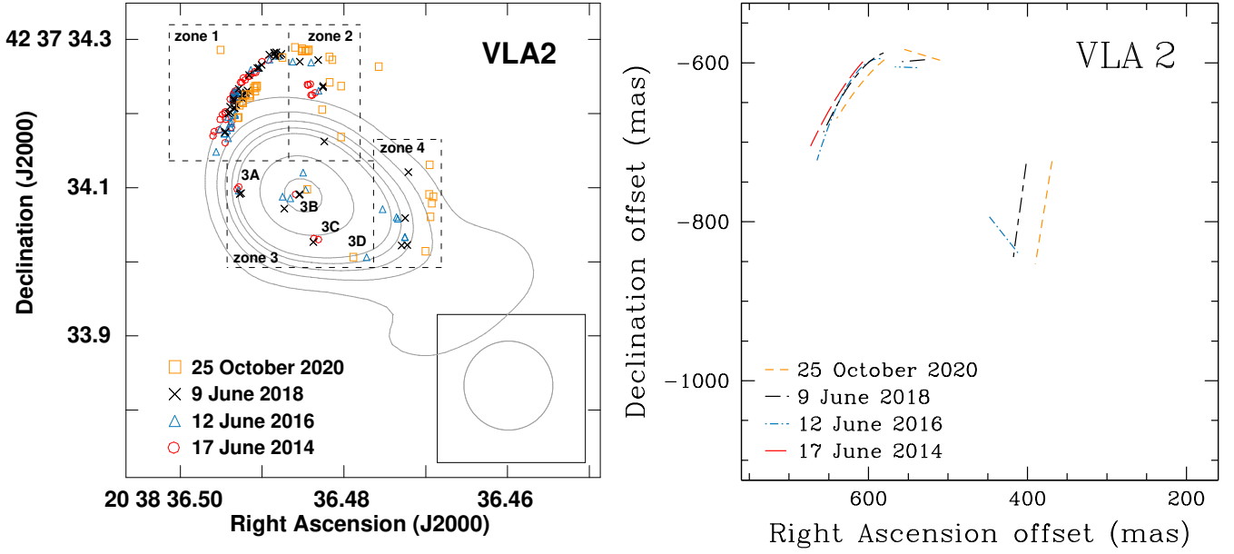
Fig. 4. Comparison of the \text{H}_2\text{O} maser features detected toward VLA 2 (left panel) in the four EVN epochs (2014.46, 2016.45, 2018.44, and 2020.82) and superimposed to the natural-weighted continuum map at K -band (central frequency 22 GHz) of the thermal, collimated ionized wind emitted by VLA 2 obtained with the VLA by Carrasco-González et al. (2015). The light gray contours are 5, 10, 15, 20, 25, 50, and 75 times \sigma = 10 \mu\text{Jy beam}^{-1} and the VLA beam is shown on the bottom right corner. The positions of the maser features are corrected assuming the proper motion of the subregion W75N(B) equal to the median proper motion measured for the 6.7 GHz \text{CH}_3\text{OH} maser features by Rygl et al. (2012), \langle \mu_\alpha \rangle = (-1.97 \pm 0.10) \text{ mas yr}^{-1} and \langle \mu_\delta \rangle = (-4.16 \pm 0.15) \text{ mas yr}^{-1} . The size of the symbols are ten times the uncertainties of the absolute positions of the maser features (see Table 2). For clarity, we show the parabolic fit of the maser features of zone 1 and the linear fit of the maser features of zone 2 (north features) and zone 4 for each epoch (right panel). The reference position is \alpha_{2000} = 20^{\text{h}}38^{\text{m}}36^{\text{s}}.43399 and \delta_{2000} = +42^{\circ}37'34''.8710 . The parameters of the linear and parabolic fits are reported in Tables 4 and 5, respectively.
