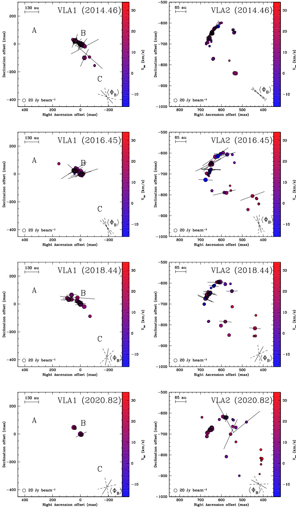
Fig. A.1. Close-up view of the 22 GHz \text{H}_2\text{O} maser features detected around the radio sources VLA 1 (left panels) and VLA 2 (right panels) in epochs 2014.46 (top panels), 2016.45, 2018.44, and 2020.82 (bottom panels). The reference positions are reported in Table 2. The letters A, B, and C indicate the position of the three maser groups identified around VLA 1 by S11a and they are reported here only for reference. The octagonal symbols are the identified maser features scaled logarithmically according to their peak intensity (Tables A.1-A.8). Maser LSR radial velocities are indicated by color (the assumed systemic velocity of the region is V_{\text{lsr}} = +10.0 \text{ km s}^{-1} ; Shepherd et al. 2003). The linear polarization vectors, scaled logarithmically according to the polarization fraction P_l , are overplotted. In the bottom-right corner of all panels the error-weighted orientation of the magnetic field ( \langle \Phi_B \rangle ) is also reported; the two dashed segments indicate the uncertainties.
