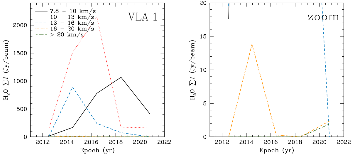
Fig. 7. Comparison of the total sum of the \text{H}_2\text{O} maser intensity ( I ) for five different ranges of velocities in VLA 1 as measured in epochs 2012.54 (VLBA, S14), 2014.46 (EVN), 2016.45 (EVN), 2018.44 (EVN), and 2020.82 (EVN).
