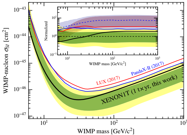
FIG. 5. 90% confidence level upper limit on \sigma_{\text{SI}} from this work (thick black line) with the 1\sigma (green) and 2\sigma (yellow) sensitivity bands. Previous results from LUX [6] and PandaX-II [7] are shown for comparison. The inset shows these limits and corresponding \pm 1\sigma bands normalized to the median of this work's sensitivity band. The normalized median of the PandaX-II sensitivity band is shown as a dotted line.
