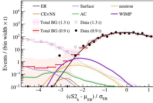
FIG. 4. Background and 200 GeV/ c^2 WIMP signal best-fit predictions, assuming \sigma_{SI} = 4.7 \times 10^{-47} \text{ cm}^2 , compared to DM search data in the 0.9 ton (solid lines and markers) and 1.3 tons (dotted lines and hollow markers) masses. The horizontal axis is the projection along the ER mean ( \mu_{ER} ), shown in Fig. 3, normalized to the ER 1\sigma quantile ( \sigma_{ER} ). Shaded bands indicate the 68% Poisson probability region for the total BG expectations.
