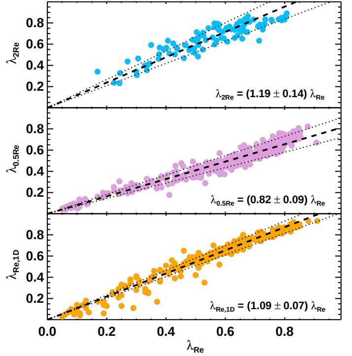
Fig. 2 Stellar angular momentum ( \lambda_R ) aperture relations for different aperture sizes. Top and middle panels show the relation between \lambda_{Re} with the values of smaller/larger apertures 0.5 R_e and 2 R_e . The bottom panel presents the comparison of \lambda_{Re} with that computed with a 1D long-slit along the major axis of the galaxies. The dashed lines indicate the biweight mean values while dotted lines the standard deviation.
