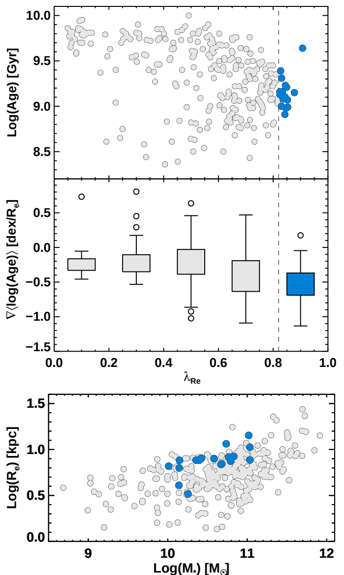
Fig. 6 (Top and middle panels) \lambda_{\text{Re}} relations with mean age within R_e , mean stellar age gradient within R_e for our sample of CALIFA galaxies. (Bottom panel) Stellar mass — size relation. The whisker plot in the middle panel was computed in the same way as in Fig. 5. Galaxies above the 95% percentile of \lambda_{\text{Re}} distribution of the sample are marked in blue. The dashed line in the top and middle panels marks that percentile.
