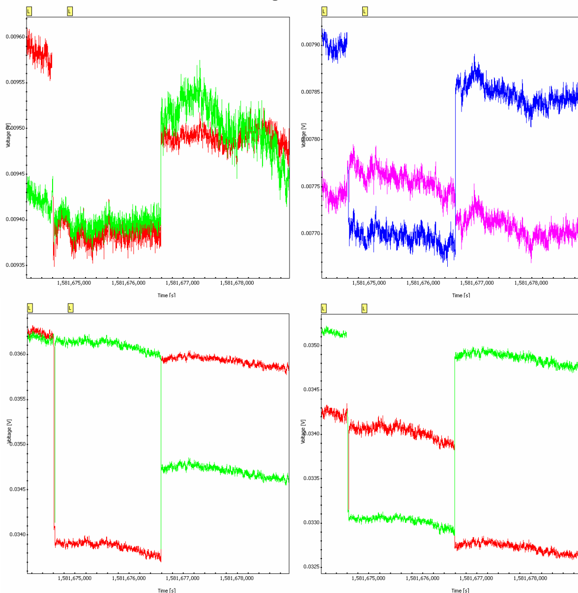
Figure 14 Channel RCA25-10 on the left and RCA25-11 on the right. RCA25-00 below Sky ref signals are not well separated when the B/D 4KHz is switched ON and further when the AC polarization is changed from 0 to 1. The same does not appear on channel 11, sharing the Hybrid, nor in the channel (R0D0) sharing the A/C 4KHz
