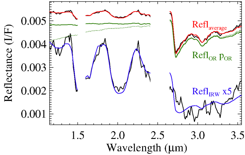
fig. S4. Model of the average spectrum as a sum of outer region signal and ice-rich wall signal. L1 observation, from the top: \text{Repl}_{\text{average}} = average spectrum (black), and the modeled best fit (red); \text{Repl}_{\text{OR}} \cdot p_{\text{OR}} = modeled reflectance of outer regions multiplied by its relative contribution to the total signal, with (green solid line) and without (green dotted line) the correction factor f discussed in Materials and Methods; \text{Repl}_{\text{IRW}} (reflectance of shadowed ice-rich wall) = \text{Repl}_{\text{average}} - \text{Repl}_{\text{OR}} \cdot p_{\text{OR}} , of both measured spectrum (black) and model (blue). Here it is multiplied by a factor of 5 for the sake of clarity.
