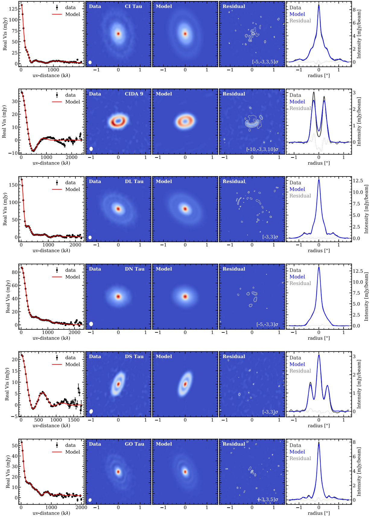
Figure 12. Comparison of data and best-fit model for individual disk, including binned and deprojected visibility profile, continuum images (data, model, and residual maps), and radial profile along the disk major axis.
