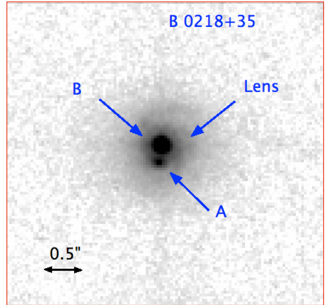
Figure 1. HST ACS WFC image of B0218+35 (filter F814W). The double point-like source is clearly detected surrounded by an extended nebula attributed to the lensing galaxy. The separation between the two sources (A and B) is \sim 0.3 arcsec.
