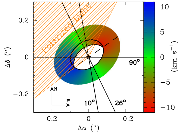
Figure 5. Synthetic OH velocity map. The dashed line shows the position angle of the disk's major axis ( 145^\circ , Ardila et al. 2007). The slit position angles at the three epochs are also shown. The dashed region shows the side of the disk which appears brighter in polarized light from Quanz et al. (2011) and Avenhaus et al. (2014).
