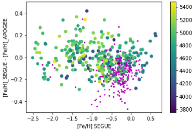
Figure 14. SEGUE vs. APOGEE [Fe/H] comparison. Dwarfs are shown as small magenta points, giants larger points color-coded by T_{\text{eff}} . The comparison sample for giants spans a large range of [Fe/H] and T_{\text{eff}} over which the offset is -0.06 and the scatter 0.15 dex. The only dwarf stars common between the surveys are metal rich and suggest that SSPP underestimates [Fe/H] for solar-metallicity dwarfs; see discussion of Figure 9.
