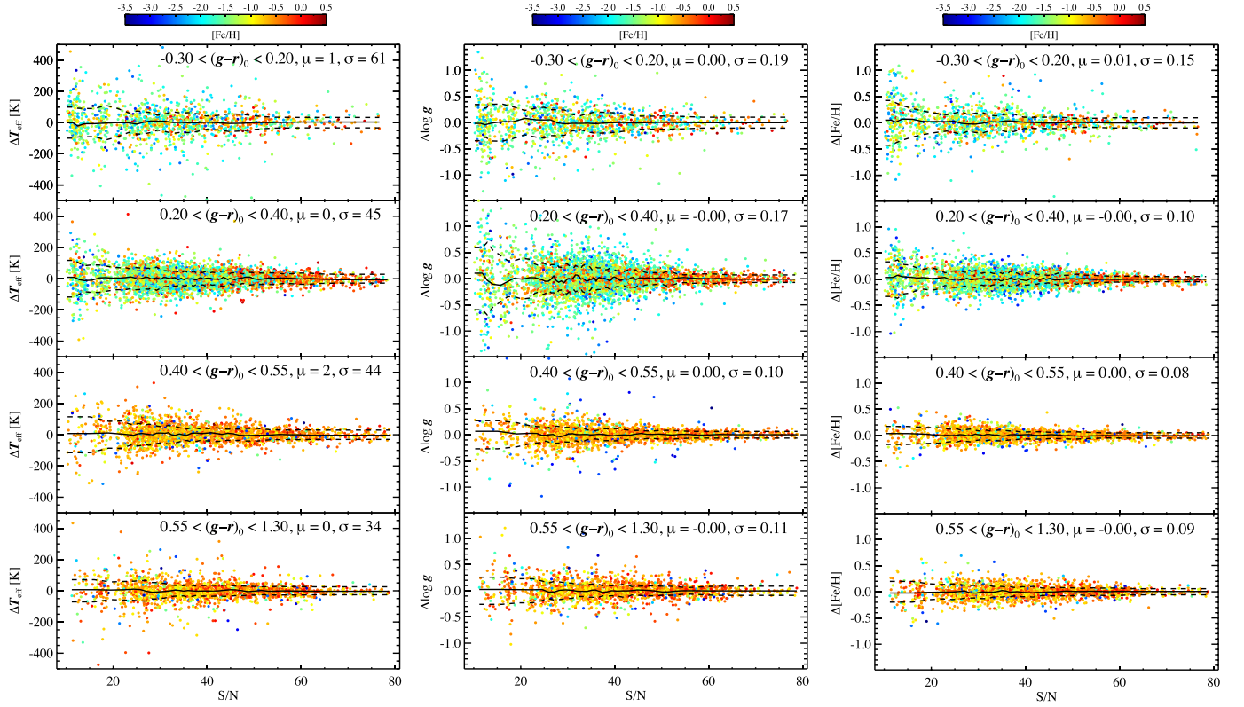
Figure 10. Residual distribution of T_{\text{eff}} , \log g , and [\text{Fe}/\text{H}] for repeat observations as a function of S/N. The sample of repeat observations is split into four different regions of (g-r)_0 . The (g-r)_0 color range in the panels runs from blue at the top to red at the bottom. The dashed line denotes one Gaussian sigma as computed for bins of 200 stars ordered by S/N. See also Table 7.
