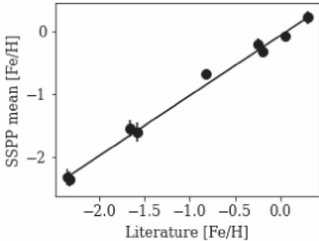
Figure 12. Summary of SEGUE SSPP cluster sample [\text{Fe}/\text{H}] measurements compared with literature values. The literature values are as given in the left panels of Figure 11. The SSPP-measured mean [\text{Fe}/\text{H}] values for the SEGUE cluster sample are given in the right panels of Figure 11. The vertical error bars are the size of the standard deviation of the [\text{Fe}/\text{H}] measurements for the SEGUE sample, also shown in the right panels. There is no systematic trend in the comparison over the entire metallicity range of the cluster sample.
