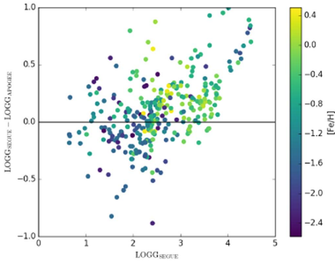
Figure 13. SEGUE vs. APOGEE log g comparison. Because ASPCAP DR14 did not provide calibrated values for dwarf stars, there are few stars in the sample with SSPP log g > 4 , and those must have large differences between ASPCAP and the SSPP to make it into the sample. Therefore, we focus our attention on the comparison with the subgiant and giant log g measurements, where the mean offset is small. The SSPP log g values are useful for separating giants from dwarfs but not as accurate as the estimates from the higher-resolution APOGEE data. See also the discussion of Figure 9.
