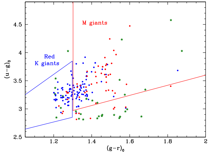
Figure 6. (u - g)_0 vs. (g - r)_0 diagram illustrating the overlap between K and M giants in their respective target types. Spectroscopically confirmed K giants are shown with blue symbols, M giants with red, and carbon stars as green stars.
