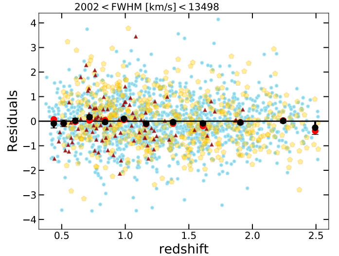
Fig. 17. Distribution of the Hubble diagram residuals (middle panel of Fig. 9) as a function of redshift for the quasars with a broad ( \text{FWHM} > 2000 \text{ km s}^{-1} ) component of the Mg II emission line in the clean sample. The black and red points represent the mean and median of the residuals in narrow redshift intervals, respectively. Symbol keys as in Fig. 1.
