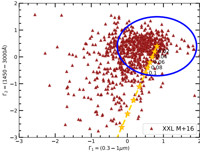
Fig. 7. Example of the \Gamma_1 - \Gamma_2 distribution for the XXL quasar sample, where \Gamma_1 and \Gamma_2 are the slopes of a power law in the \log(\nu) - \log(\nu L_\nu) plane in the 0.3-1\mu\text{m} and 1450-3000\text{\AA} intervals, respectively (see Sect. 7.1). The stars represent the \Gamma_1 - \Gamma_2 values of the quasar SED by Richards et al. (2006) with increasing dust reddening (following the extinction law of Prevot et al. 1984), with E(B - V) in the range 0-0.3 . We selected all the quasars inside the blue circle (i.e. with minimum host-galaxy and dust reddening contamination).
