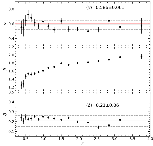
Fig. 8. Redshift evolution of the slope \gamma , the intercept \hat{\beta} and the dispersion \delta of the F_X - F_{\text{UV}} relation. To perform the regression fit, X-ray and UV fluxes have been normalised to 10^{-28} and 10^{-30} \text{ erg s}^{-1} \text{cm}^{-2} \text{Hz}^{-1} , respectively. The data points in each panel are averages in narrow redshift bins ( \Delta z \approx 0.06 - 0.45 ). Error bars represent the 1\sigma uncertainty on the mean in each bin. The grey solid and dashed lines are the means and 1\sigma uncertainties, respectively, on the slope ( \gamma ) and on the dispersion ( \delta ). The red line marks \gamma = 0.6 .
