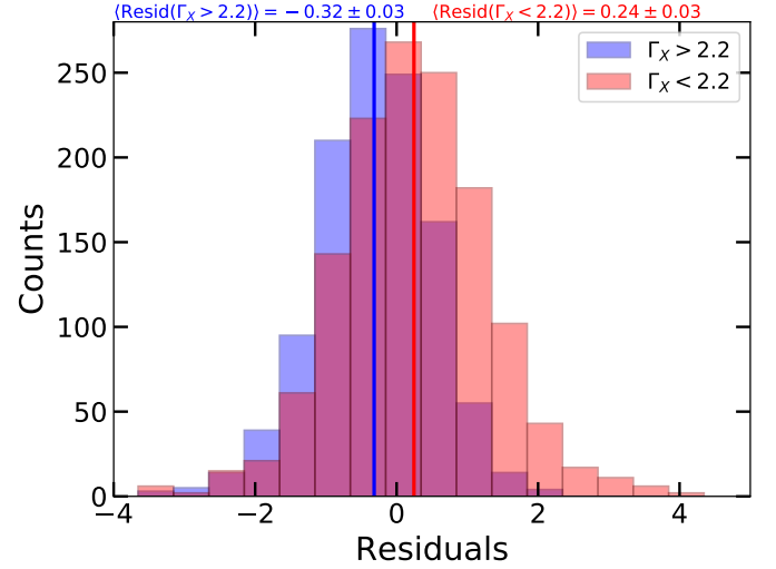
Fig. 14. Distribution of the Hubble diagram residuals (middle panel of Fig. 9) for the quasars with \Gamma_X higher (blue) and lower (red) than the average (i.e. \langle \Gamma_X \rangle = 2.2 , see Fig. 12). The blue and red solid lines represent the mean of the residuals in each \Gamma_X distribution, respectively (averages are reported on top).
