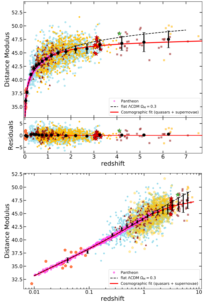
Fig. 9. Top panel: distance modulus–redshift relation (Hubble diagram) for the clean quasar sample and supernovae Ia ( Pantheon , magenta points). Symbol keys are the same as in Fig. 1. The red line represents a fifth order cosmographic fit of the data, whilst the black points are averages (along with their uncertainties) of the distance moduli in narrow (logarithmic) redshift intervals. The dashed black line shows a flat \Lambda CDM model fit with \Omega_M = 0.3 . Middle panel: residuals with respect to the cosmographic fit and the black points are the averages of the residuals over the same redshift intervals. Bottom panel: distance modulus–redshift relation plotted with a logarithmic horizontal axis scale to better visualise the agreement between supernovae Ia and quasars in the low-redshift range.
