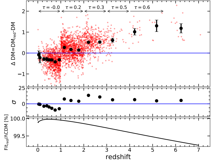
Fig. 16. Analysis of the possible contribution of dust at 2500 Å. Top: distribution of the difference of the distance moduli ( \Delta DM , red points; \Delta DM = 0 represents the \Lambda CDM) as a function of redshift. The parameter \Delta DM is defined as DM_{\text{red}} - DM , where DM is computed from the quasar data as described in Sect. 9. The DM_{\text{red}} values are estimated by correcting the observed F_{UV} for an additional intrinsic (and redshift-dependent) extinction. \tau is the optical depth at the rest-frame 2500 Å that would be needed to ascribe the discrepancy to an underestimated dust extinction in the UV flux. The black points represent the average (and 1\sigma uncertainties) of \Delta DM in the same narrow redshift intervals used in Figs. 8 and 9. Middle: deviation in \sigma of the average points with respect to \Lambda CDM. Bottom: ratio between the cosmographic fit obtained from the data, where F_{UV} is corrected for additional extinction, and the \Lambda CDM. The cosmographic fit perfectly matches \Lambda CDM for the chosen values of dust reddening (see Sect. 11.4).
