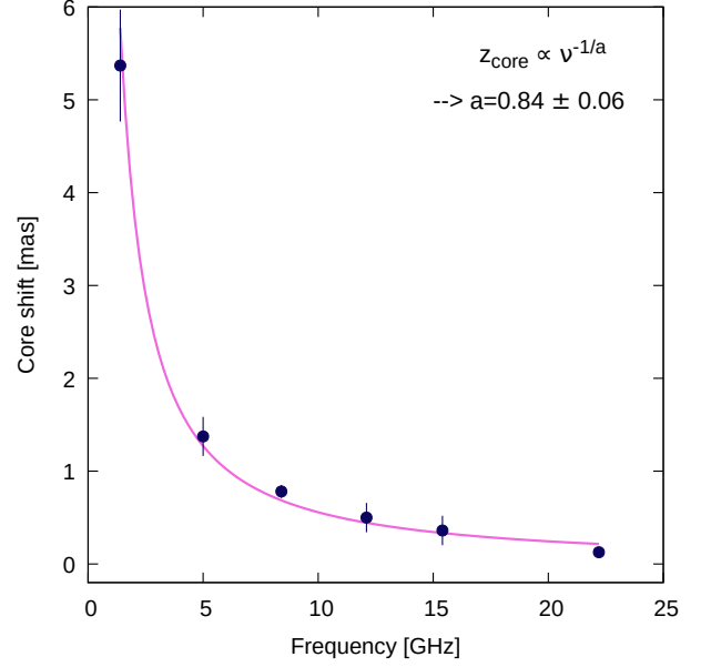
Fig. 2. Core positions as a function of frequency relative to the mm-VLBI cores (43 GHz and 86 GHz).
