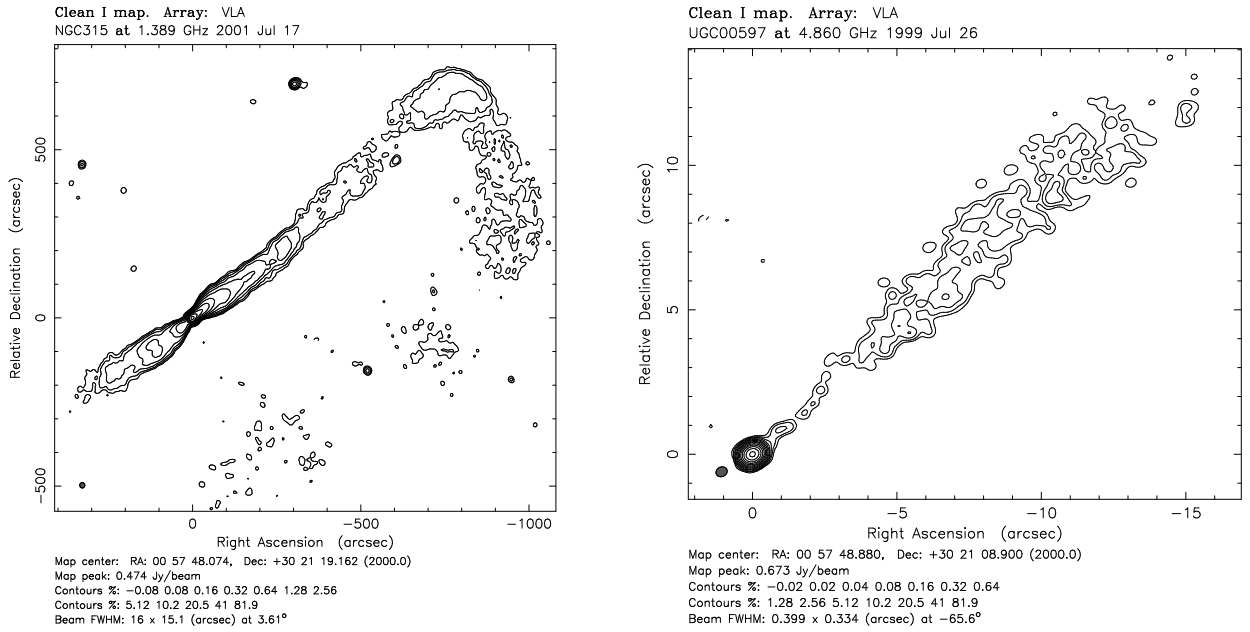
Fig. .8. VLA images of NGC 315 at 1 GHz (left) and 5 GHz (right).
