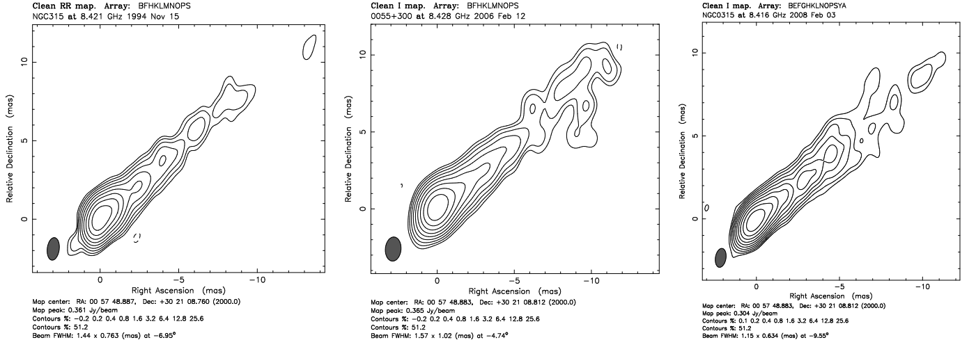
Fig. 3. VLBI images of NGC 315 at 8 GHz.
