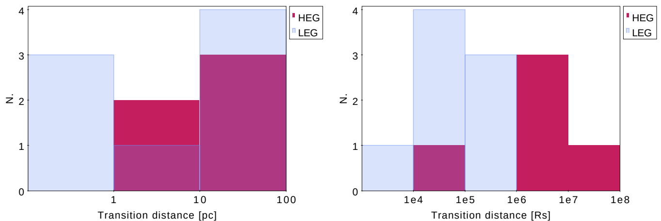
Fig. 6. Distribution of the de-projected transition distance in low-excitation (LEG) and high-excitation (HEG) galaxies. Left panel: the distance is expressed in units of parsecs. Right panel: the distance is expressed in units of Schwarzschild radii.
