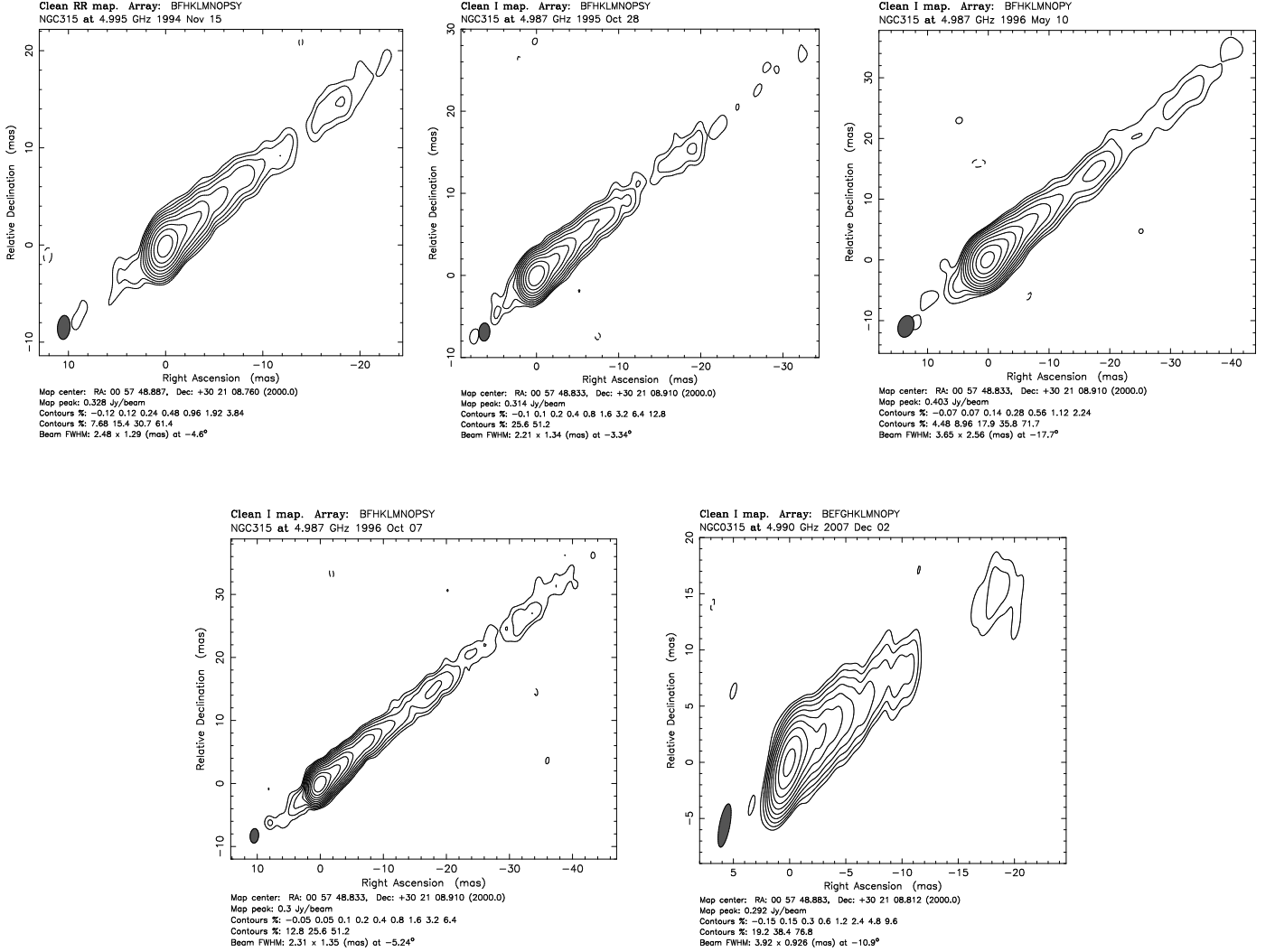
Fig. .2. VLBI images of NGC 315 at 5 GHz.
