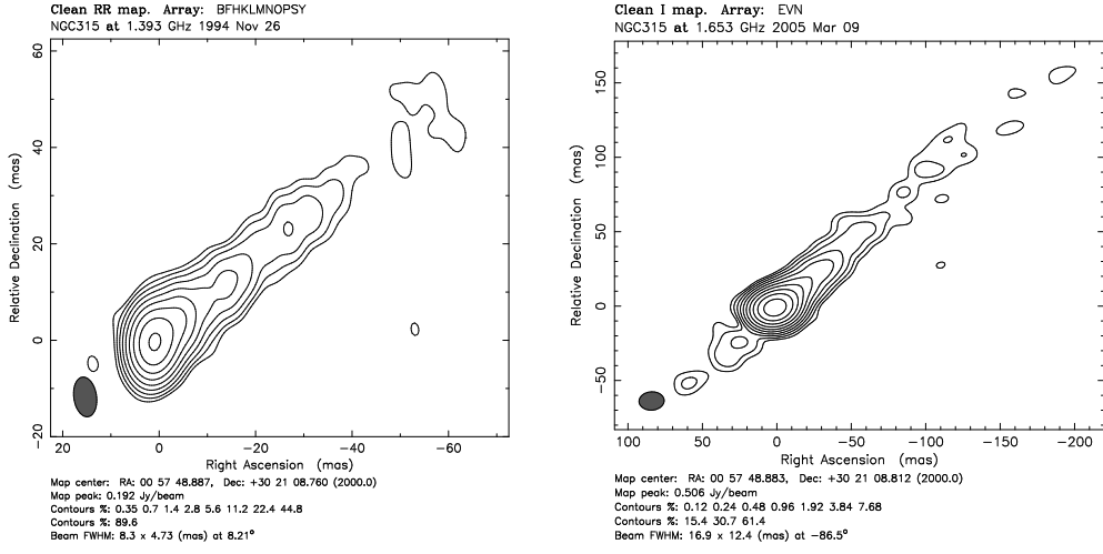
Fig. .1. VLBI images of NGC 315 at 1 GHz.
