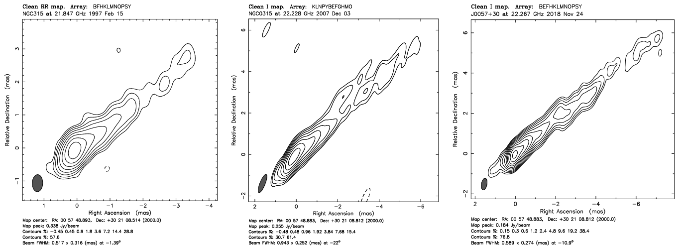
Fig. 5. VLBI images of NGC 315 at 22 GHz.
