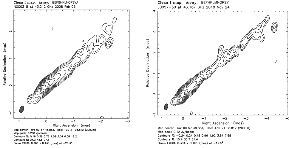
Fig. .6. VLBI images of NGC 315 at 43 GHz.
