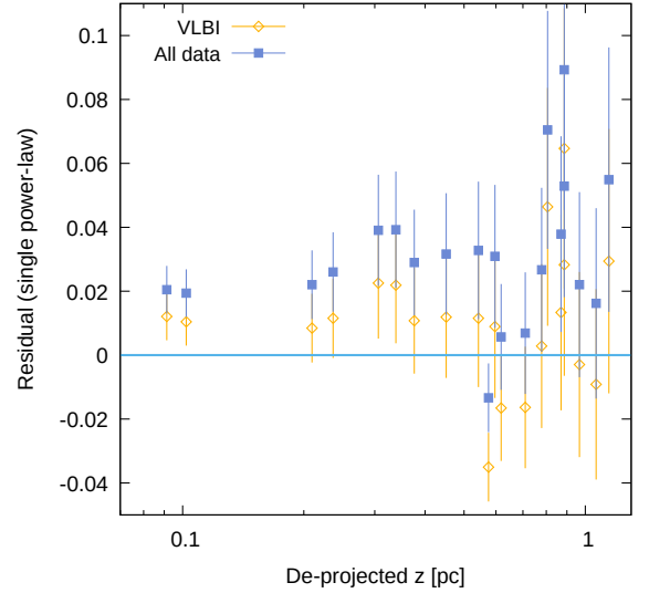
Fig. 4. Residuals in the innermost jet region for a single power-law fit performed considering the VLBI data only and the entire data set (VLBI+VLA).
