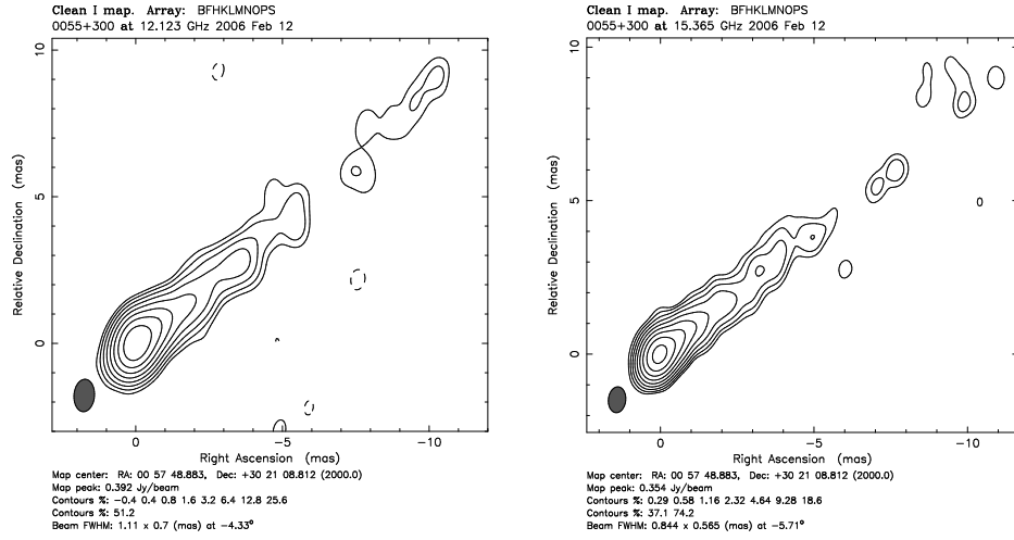
Fig. 4. VLBI images of NGC 315 at 12 GHz (left) and 15 GHz (right).
