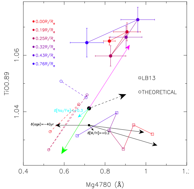
Figure A3. Same as in Fig. 8 but plotting TiO0.89 as a function of the Mg4780 IMF-sensitive feature. The cyan arrow shows the sensitivity of Mg4780 on [\text{Na}/\text{Fe}] , based on CvD12 SSP models.
