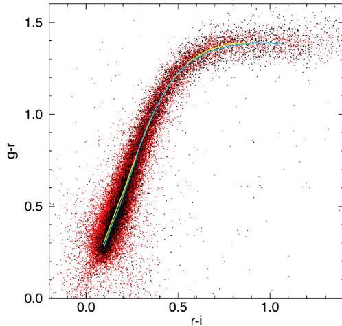
Figure 3. Colour–colour ( g - r, r - i ) diagram showing a sample of stars from ShaSS (black dots) overimposed on a sample of SDSS stars (red dots). The curves trace the loci of the stars in the plane (ShaSS: cyan; SDSS: yellow). The distance between the curves never exceeds \sim 0.015 mag.
