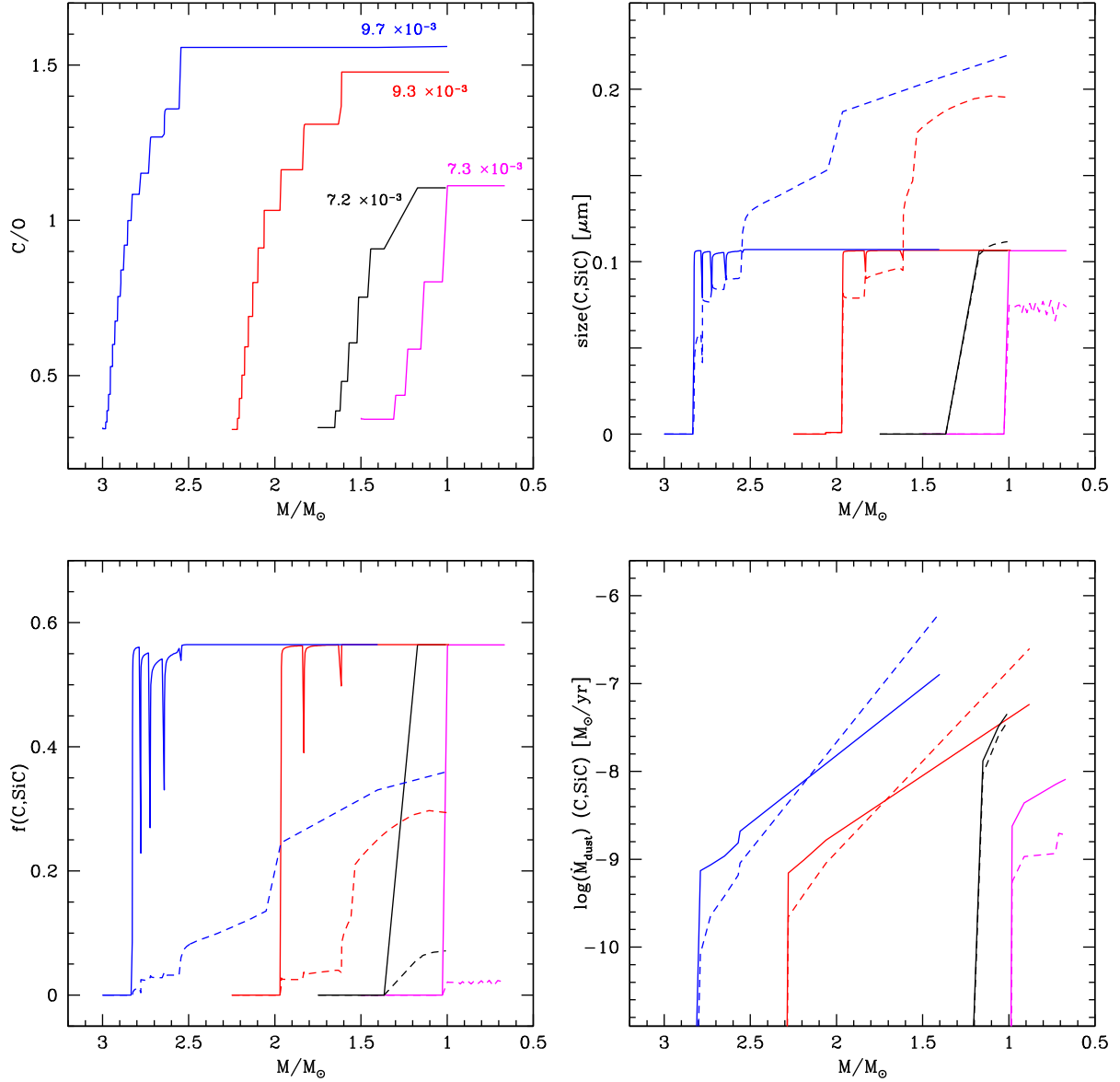
Figure 3. Variation during the AGB phase of the physical and dust properties of stars with initial mass in the range [1.5–3] M_{\odot} , shown by the coloured lines from magenta to blue. The current mass of the star (decreasing during the evolution) is displayed on the abscissa. The quantities shown in the four panels are: surface C/O ratio, with the values of the final surface carbon mass fraction also indicated (top-left), size of SiC and solid carbon grains (top-right, solid and dashed lines, respectively), fraction of silicon condensed into SiC and of carbon condensed into dust (bottom-left, solid and dashed lines, respectively), SiC and carbon mass-loss rates (bottom-right, solid and dashed lines, respectively). A coloured version of this plot is available online.
