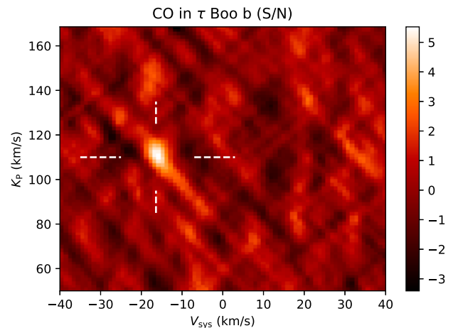
Figure 8. CO signal obtained by cross-correlating VLT/CRIRES spectra of exoplanet \tau Boötis b around 2.3 \mu\text{m} with a CO model matching the best-fitting parameters of Brogi et al. (2012). The cross-correlation signal is shown as function of systemic velocity V_{\text{sys}} and maximum orbital radial velocity K_p . The known values of (-16.4, 110) km s -1 are marked with dashed white lines and are a good match to these observations.
