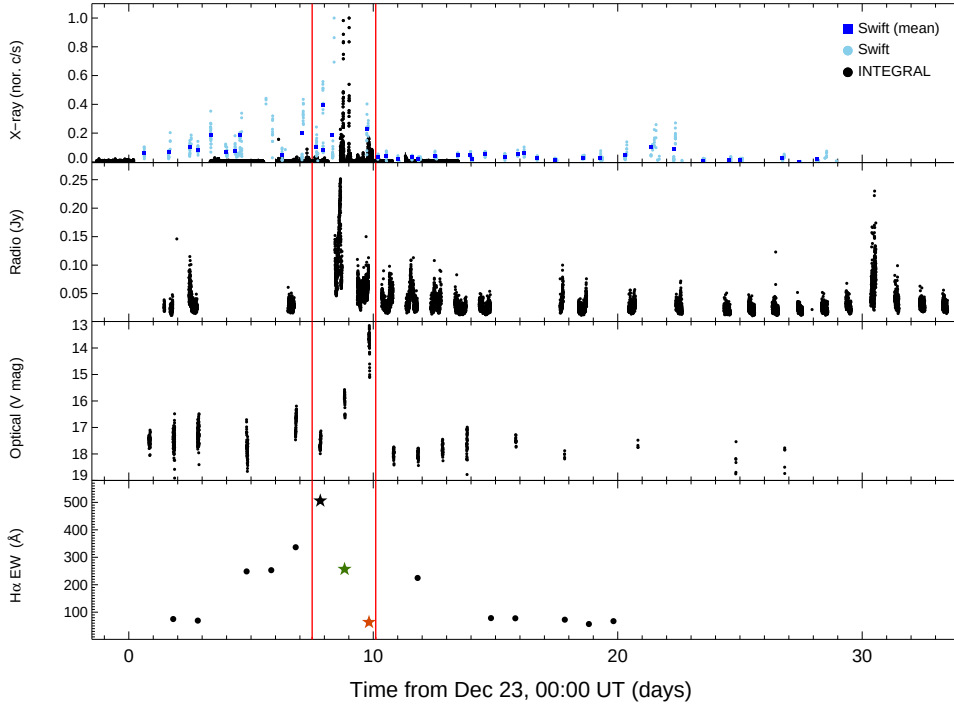
Figure 1. From top to bottom X-ray (Swift and INTEGRAL), radio and optical lightcurves covering the December 2015 (to January 2016) mini-outburst of V404 Cyg. The bottom-most panel shows the H\alpha EW evolution derived from GTC and WHT spectra. The two vertical lines encompass the interval of highest activity, where conspicuous wind signatures are present in the spectra (marked as stars).
