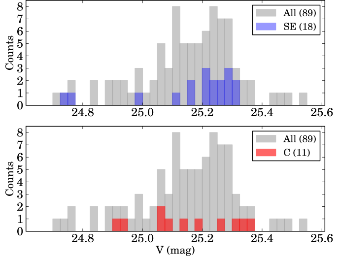
Fig. 15.— Lower panel : Distribution in apparent V mean magnitude of the 11 RR Lyrae stars in the C region. Upper panel : Same as in the lower panel, but for the 18 RR Lyrae stars in the SE region.
