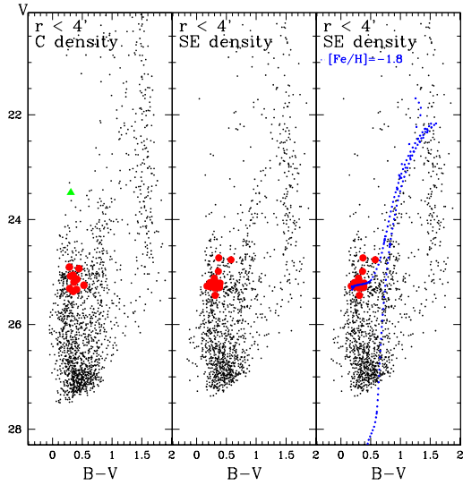
Fig. 14.— Left : CMD of sources in the C over-density region. Center : Same as in the left panel, but for the SE region. Right : CMD of the SE region with superimposed an isochrone of 13 Gyr with [Fe/H] = -1.8 dex (blue dotted line; see text for details).
