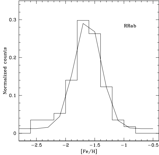
Fig. 6.— Metallicity distribution of And XXVII RRab stars obtained using Alcock et al.(2000) method. The distribution peaks at [\text{Fe}/\text{H}] \sim -1.62 with \sigma \sim 0.23 dex.
