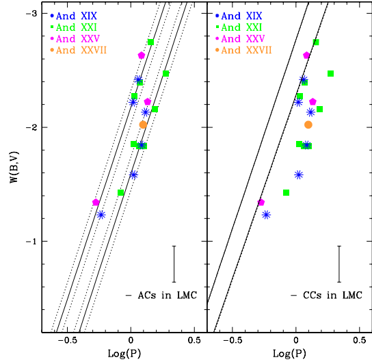
Fig. 7.— Position on the PW plane of star V2 (orange filled circle). Solid lines represent the PW relations for ACs (left panel; Ripepi et al. 2014) and CCs in the LMC (right panel; Jacyszyn-Dobrzniecka et al. 2016), respectively. Blue, green and magenta symbols are ACs we have identified in And XIX (Paper I), And XXI (Paper II), and And XXV (Paper III). The dotted lines show the \pm 1\sigma deviations. For the CCs the errors of the fits are very small and the confidence contours are very close to the fits.
