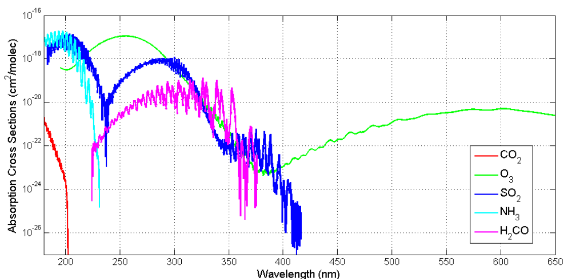
Figure 1: Absorption cross sections of \text{CO}_2 , \text{H}_2\text{CO} , \text{NH}_3 , \text{SO}_2 , and \text{O}_3 considered in this study
