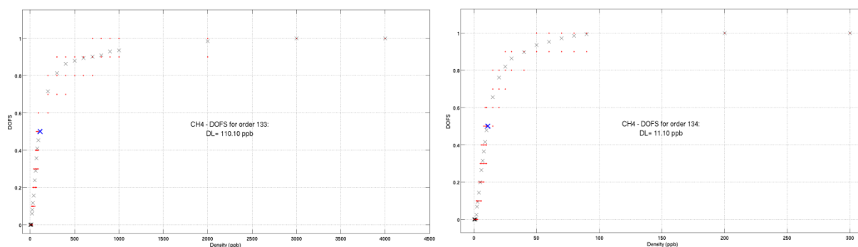
Figure 5: Degree of freedom for Signal of the retrievals in the LNO diffraction order 133 (2989.416 - 3013.415 cm -1 ) and order 134 (3011.893 - 3036.072 cm -1 ) for CH 4 . The red dots correspond to each individual retrieval. The black crosses represent the averages of the DOFS for each considered factor. The blue cross indicates the value of DOFS=0.5 hence the value of the detection limit in abscissa, in ppb.
