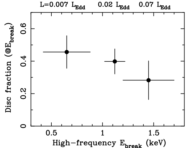
Figure 6. The energy at which a trend reversal is observed in the high-frequency lag-energy spectra (obtained fitting the spectra with a broken power law model) as compared to the disc flux fraction (i.e. the ratio between the disc and the disc-plus-power law flux) in the energy bin of the reversal.
