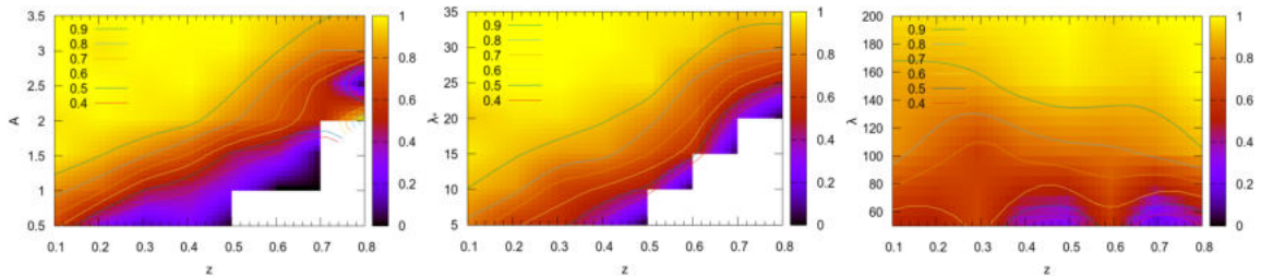
Figure 13. Left-hand panel: completeness of the cluster catalogue as a function of redshift z and amplitude A . Centre and right-hand panels: same as in the left-hand panel but for the intrinsic richness \lambda_* and the apparent richness \lambda . The iso-contours trace the completeness from 0.4 to 0.9 as indicated in the figure. Where the completeness is extremely low, there are no sufficient data (white areas).
