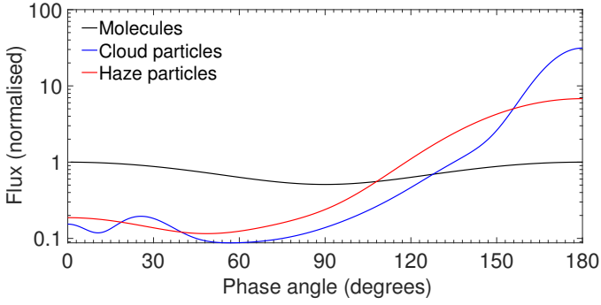
Fig. 16. Single scattering flux and linear polarisation of the cloud and haze particles at 550 nm along with Rayleigh scattering curves. The phase angle, \alpha , is 180^\circ - \Theta , where \Theta is the single scattering angle.
