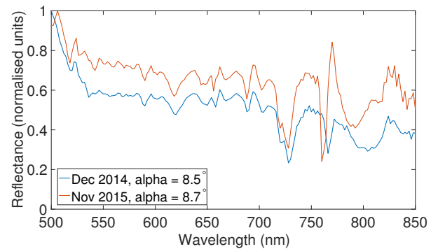
Fig. 8. Normalised reflectance spectra for the two datasets.
