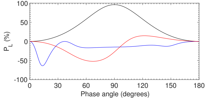
Fig. 16. Single scattering flux and linear polarisation of the cloud and haze particles at 550 nm along with Rayleigh scattering curves. The phase angle, \alpha , is 180^\circ - \Theta , where \Theta is the single scattering angle.
