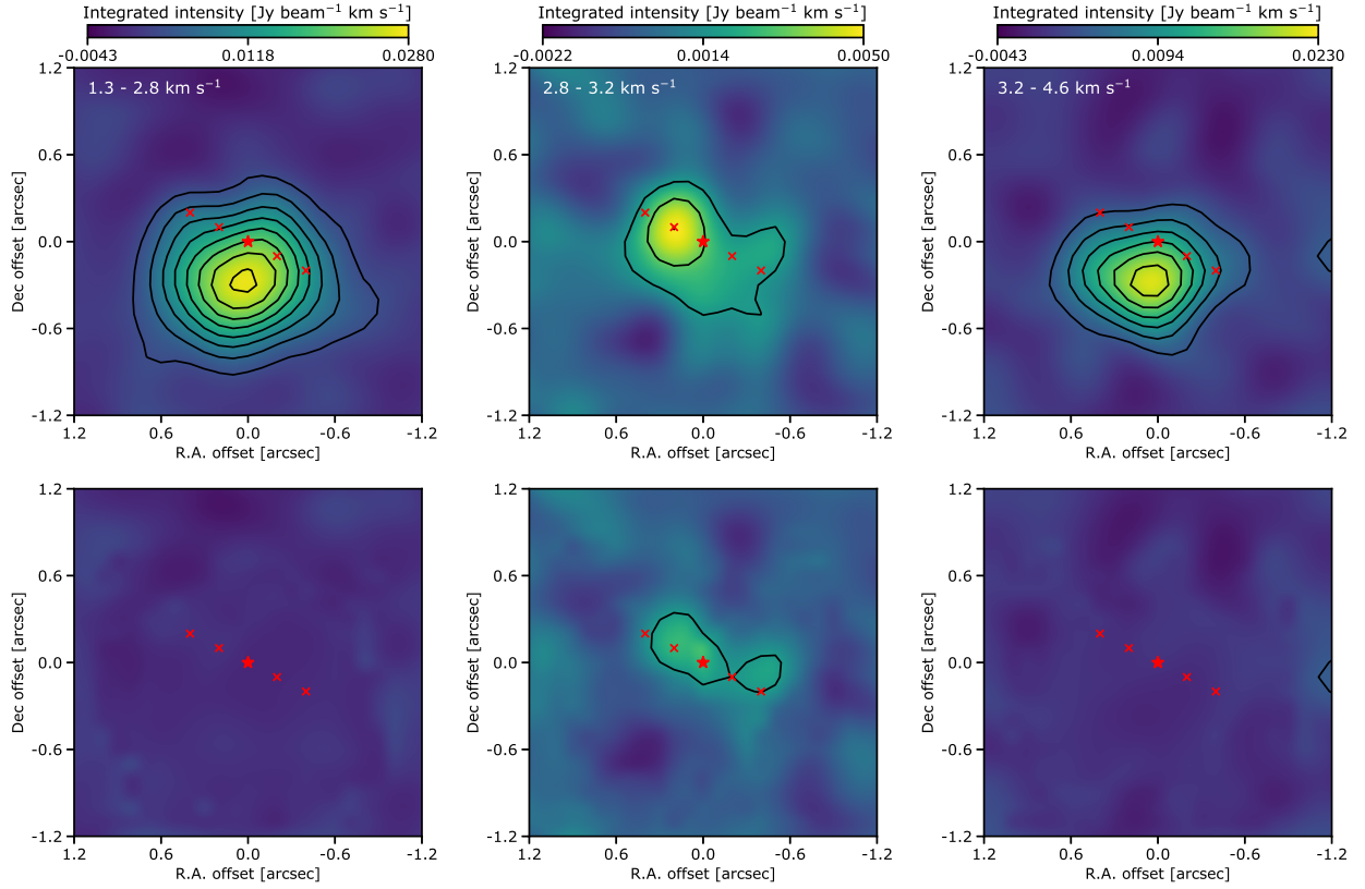
Fig. 2. Top panels: integrated intensity maps around the ^{16}\text{O}^{18}\text{O} transition at 233.946098 GHz for velocities of 1.3–2.8 (left panel), 2.8–3.2 (middle panel), and 3.2–4.6 (right panel) \text{km s}^{-1} . Bottom panels: residual maps of the integrated intensity emission after subtraction of the fit performed with the line profile of the reference transition. Contours are in steps of 3\sigma , with \sigma of 1.07, 0.54, and 1.08 \text{mJy beam}^{-1} \text{km s}^{-1} , respectively. The red star symbols depicts the position of the IRAS16293 B continuum peak while red crosses show the positions of the half-beam and full-beam offset positions mentioned in the text.
