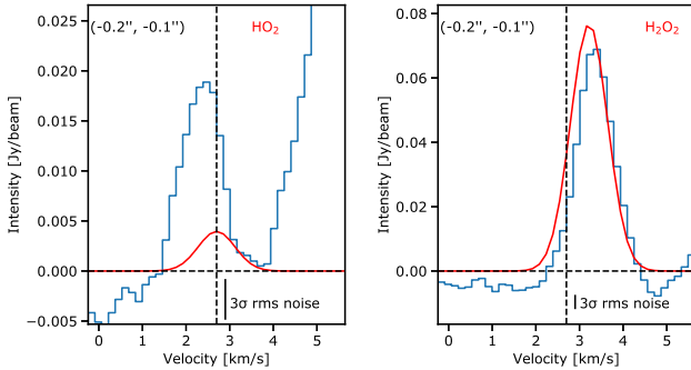
Fig. 3. Observed spectra (in blue) around the \text{HO}_2 transition at 236.280920 GHz (left panel) and around the \text{H}_2\text{O}_2 transition at 235.955943 GHz (right panel), respectively, towards the western half beam position. The red line in the left and right panels shows the modelled spectrum at LTE obtained with a \text{HO}_2 column density of 1.1 \times 10^{14} \text{cm}^{-2} and T_{\text{ex}} = 125 \text{ K} and a \text{c-C}_2\text{H}_4\text{O} column density of 6.1 \times 10^{15} \text{cm}^{-2} and T_{\text{ex}} = 125 \text{ K} , respectively (see text). Positions in arcsec relative to the continuum peak position of IRAS 16293 B are shown at the top left of each panel. The vertical and horizontal black dashed lines depict the source velocity at 2.7 \text{ km s}^{-1} and the baseline, respectively.
