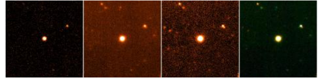
Fig. A.2. From left to right: ugi and RGB thumbnail of one UCD candidate in the \sim 1 sq. degree area centered on NGC 3115. The boxes are 1' on each side.
