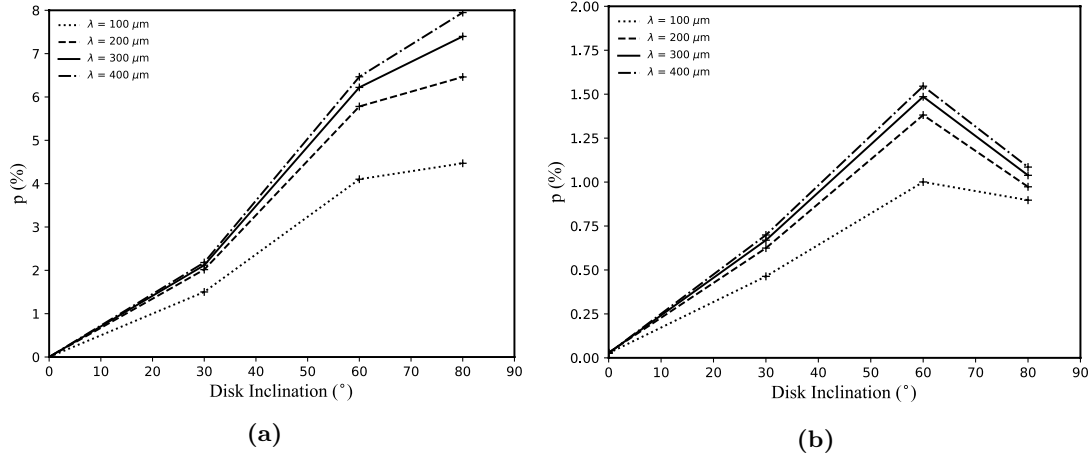
Figure 15. Spatially integrated polarization levels expected at 100–400 \mu\text{m} from magnetized protoplanetary disks as a function of disk inclination ( 0^\circ refers to a pole-on disk configuration). The left panel (a) considers a poloidal magnetic field topology, and the right panel (b) a toroidal one. See Li et al. (2016) for more details about the assumptions of the disk model and the adopted parameter values.
