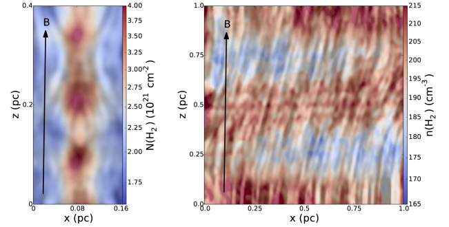
Figure 3. Simulated striations (from Tassis and Tassis 2016). Right panel: Volume density image from the simulations. Left panel: Zoomed-in column density view of a single striation, showing the “sausage” instability setting in, with characteristic imprints in both the magnetic-field and the column-density distribution. In both panels, the drapery pattern traces the magnetic field lines and the mean direction of the magnetic field is indicated by a black arrow. The passage of Alfvén waves excites magnetosonic modes that create compressions and rarefactions (colorbar) along field lines, giving rise to striations. The simulated data in both panels have been convolved to an effective spatial resolution of 0.012 pc, corresponding to the 18'' HPBW of B-BOP at 200 \mu\text{m} .
