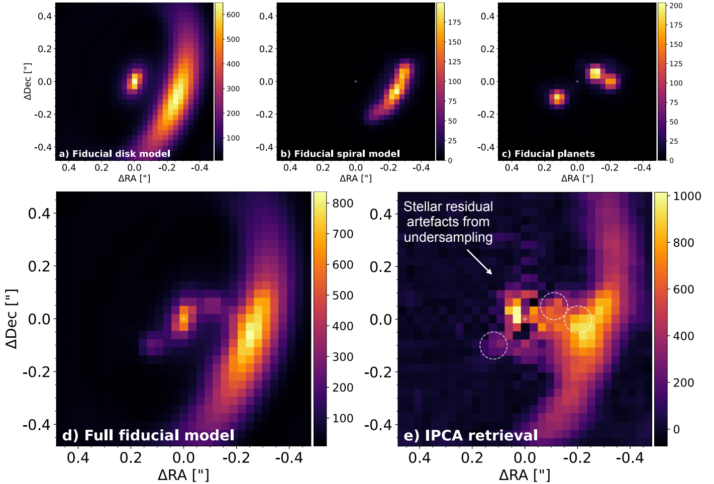
Fig. A.3. Fiducial model of the circumstellar signals of PDS 70 ( d ) compared to the image recovered by IPCA ( e ) using the same reduction parameters as for the PDS 70 dataset. The different components of the model are shown in panels a-c . This model was injected at two different roll angles separated by 5.0^\circ in the NIRCcam dataset of HD 135067 at a similar contrast as the circumstellar signals of PDS 70. The protoplanet locations are indicated with dashed circles in panel e . The recovery of all signals from the model at a similar level as injected casts confidence in the results obtained with IPCA from the PDS 70 data.
