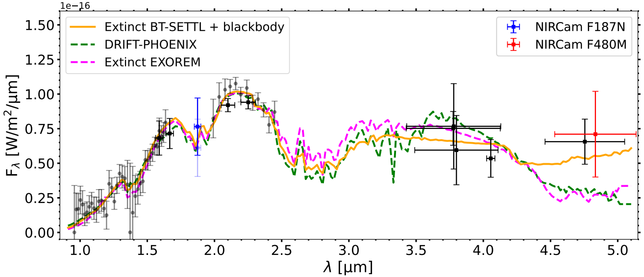
Fig. 2. Composite SED of PDS 70 b showing spectro- and photometric measurements from the literature (gray and black error bars, respectively), the new NIRCам F187N and F480M photometry (blue and red error bars, respectively), and the best-fit atmospheric models found in Wang et al. (2021b). The model with the most support is shown with a solid orange line (extinct BT-SETTL model with additional blackbody emission). It is consistent with both of our measurements, and suggests that circumplanetary contribution is required. The light blue error bar is obtained considering photometry from the literature for the star. It illustrates the uncertainty associated with variability that affects some other data points of the SED (details in Appendix F).
