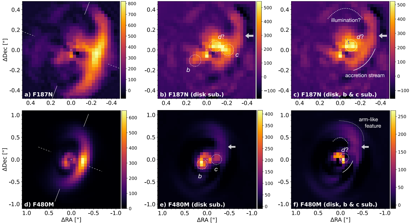
Fig. 1. NIRCам images of PDS 70 obtained in the F187N (top row) and F480M (bottom row) filters using our iterative PCA algorithm. The second and third columns show the images obtained after subtraction of our outer-disk model and after further subtraction of protoplanets b and c , respectively. The major and minor axes of the disk are indicated in the first column with solid and dashed lines, respectively. The dashed circles indicate the predicted locations of protoplanets b and c based on the orbital fits in Wang et al. (2021b) and the location of candidate d based on the orbit suggested in M19. The astrometric measurements for d (blue dots) are compared to our new estimated astrometry (solid circle) in panel c. The units are MJy sr -1 .
