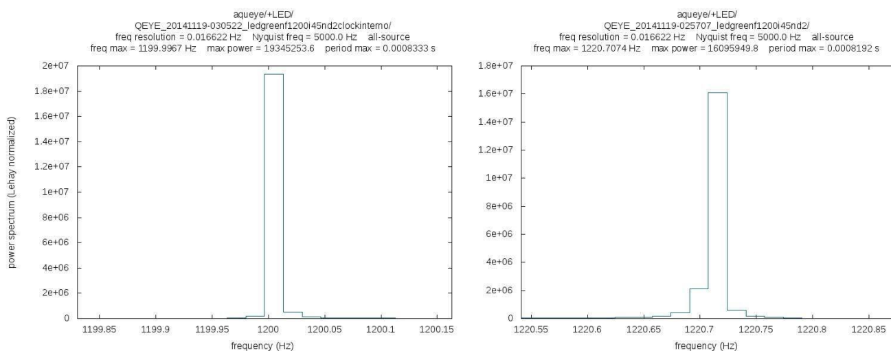
Figure 13: Enlargement around the maximum frequency of the power spectrum of an approximately square wave input signal at \sim 1200 Hz. Left : signal generated with the internal H14 Oscillator. Right : signal generated with the external Rubidium clock.
