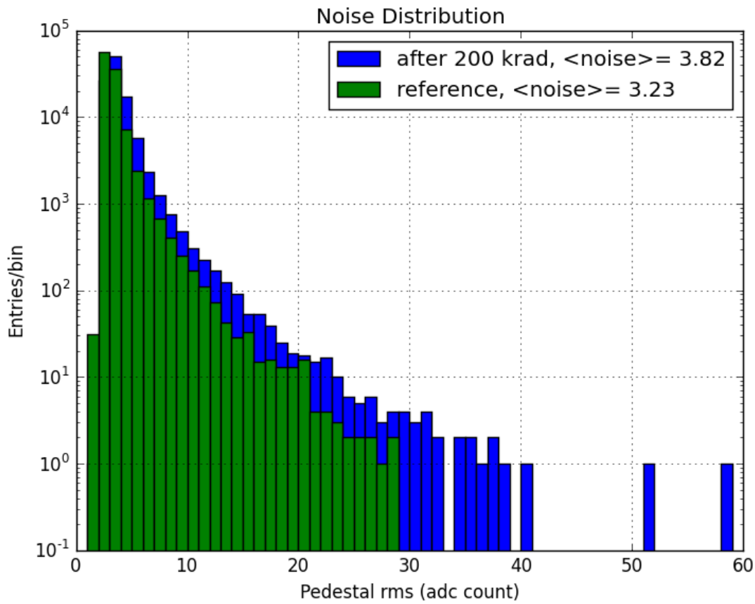
Figure 5: Variation of the electronic noise at 200 krad. The histogram in green is before starting the irradiation. The histogram in blue is at a TID level of 200 krad.
