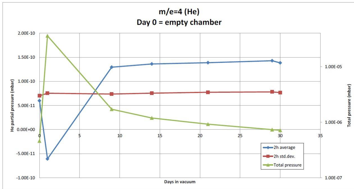
Figure 21 Averaging results for 30 days in the vacuum. Green line= chamber total pressure [mbar]; blue line= He partial pressure 2h average [mbar]; red line= He partial pressure std. dev. [mbar].
