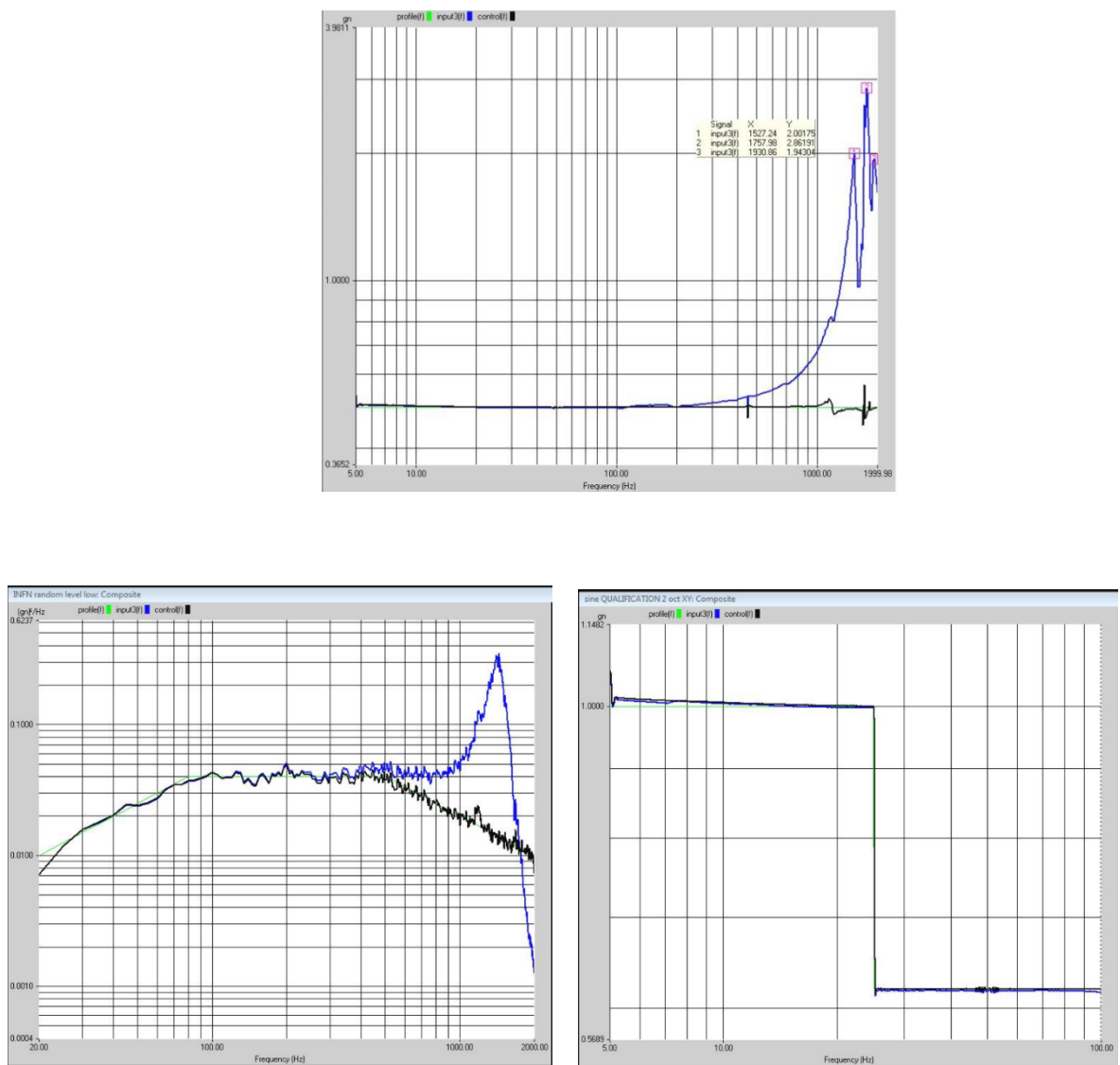
Figure 15 The sine sweep spectra, the random tests and the sinusoidal results for the X axis.
