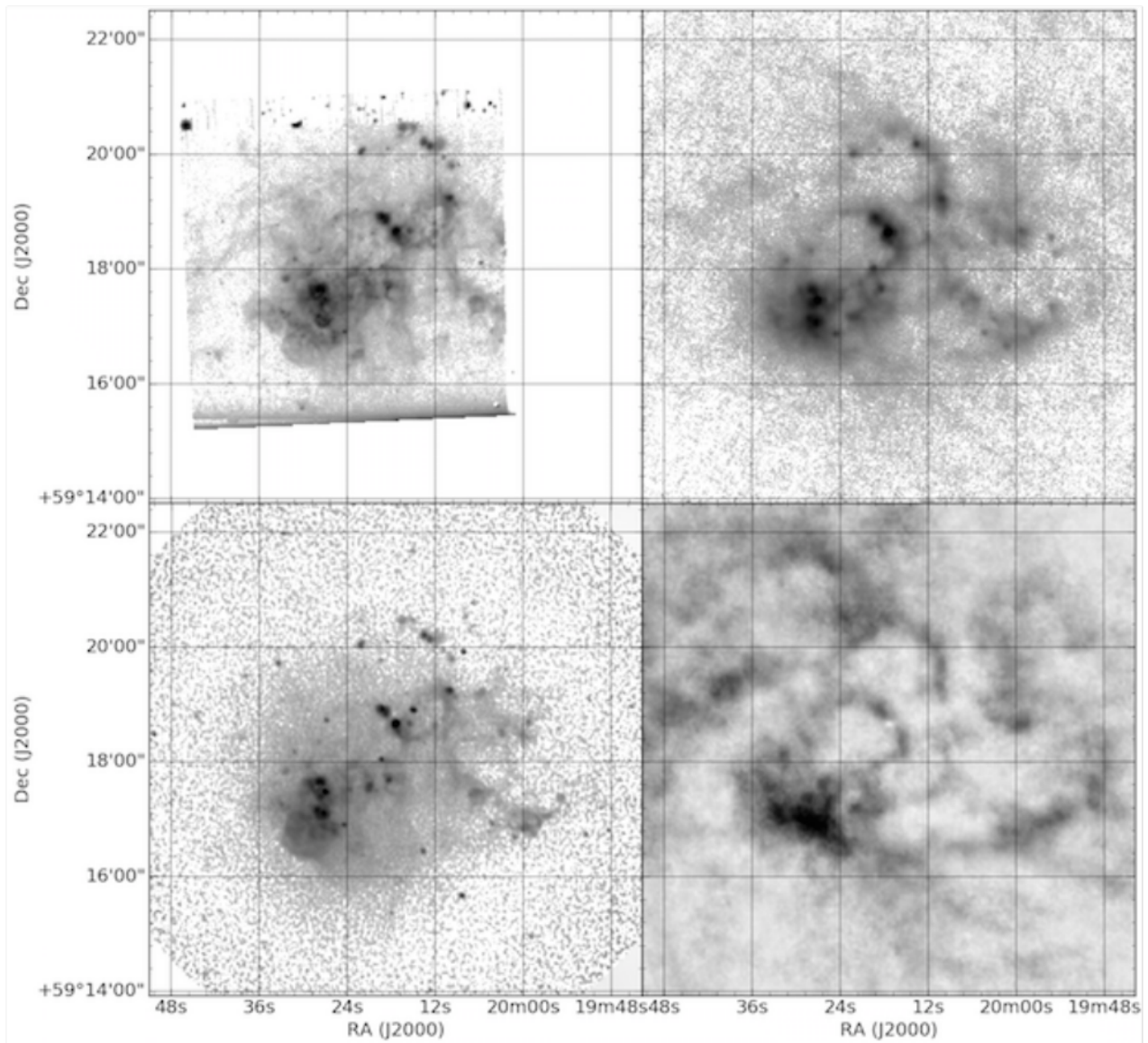
Figure 1. IC 10 at multiple wavelengths. Top Left: H \alpha continuum subtracted map taken from Hunter & Elmegreen (2004) . Top Right: Map of IC 10 at 70 \mu m taken with Herschel as part of the Dwarf Galaxy Survey ( Madden et al. 2013 ). Bottom Left: 5 GHz VLA C & D array map of IC 10 taken from Heesen et al. (2015) . Bottom Right: Naturally weighted HI map of IC 10 taken as part of LITTLE THINGS ( Hunter et al. 2012 ). Note how the large-scale holes and shells in the HI distribution can be easily identified across multiple wavelengths.
