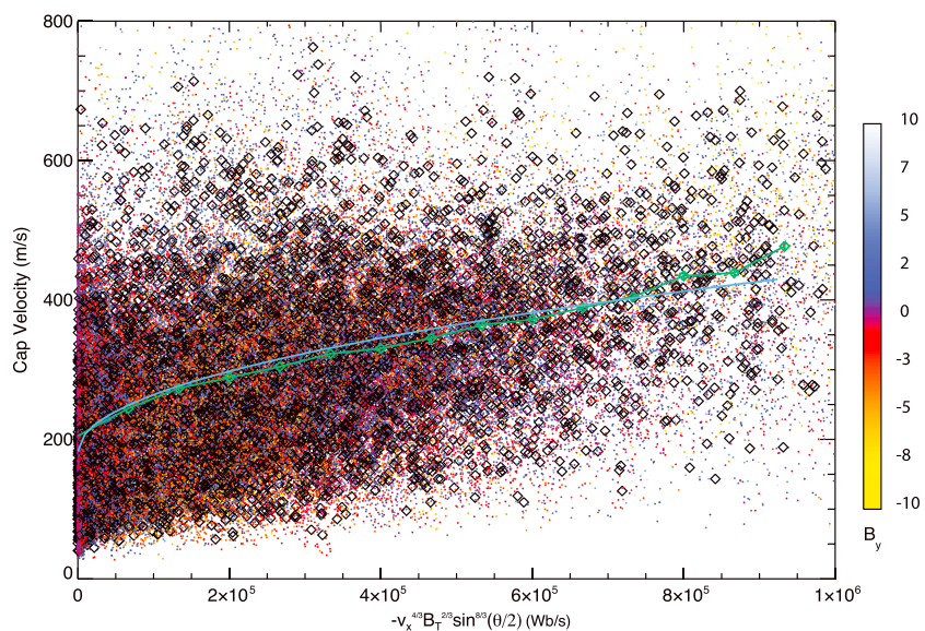
Figure 8. Scatterplot showing the observed velocity in the polar cap versus the E_{MP} parameter. Each point is an average of all measurements within the 85^\circ latitude circle. The black diamonds represent time averages over 15 min. The green diamonds and connecting line show the average value in 10 bins of E_{MP} . The blue line shows a fit of the averages versus \sqrt{E_{MP}} .
