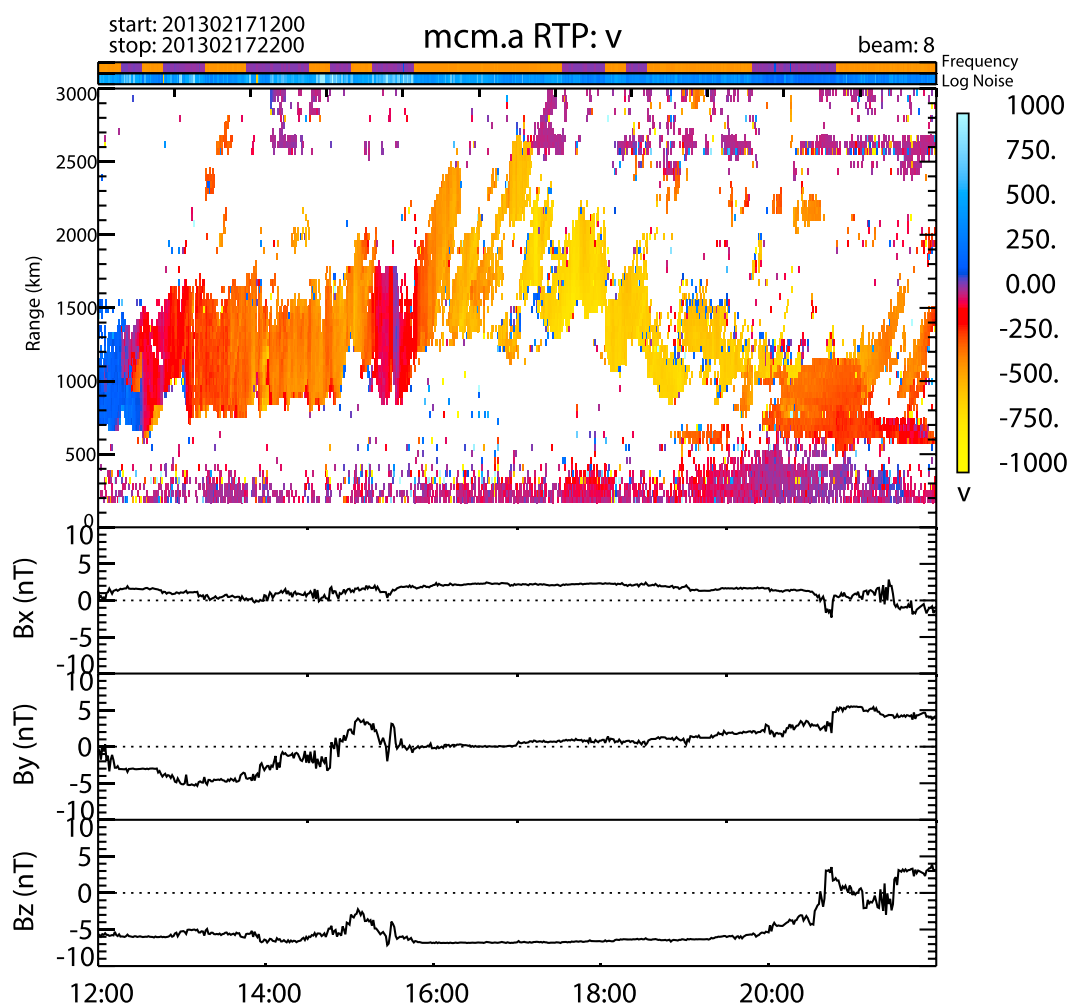
Figure 2. Range-time-velocity plot for returns observed by the McMurdo radar along its central beam and IMF observations from the ACE space form 17 February 2013 between 1200 UT and 2200 UT. Figure shows the three components B_x , B_y , and B_z in GSM coordinates. The IMF values have been time delayed to the assumed position of the magnetopause
