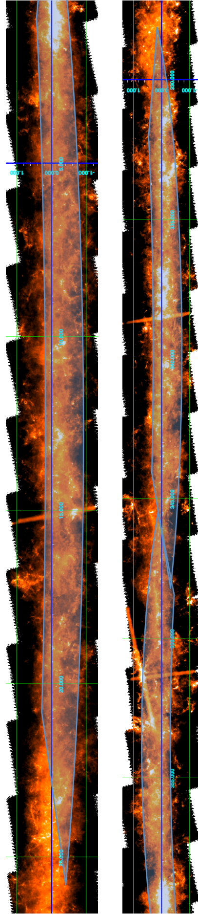
Fig. 1. b) As in Fig. 1a, but for the longitude ranges 0^\circ \leq l \leq 27^\circ ( upper panel ) and 327^\circ \leq 360^\circ ( lower panel ), encompassing the range spanned by the Galactic Bar.
