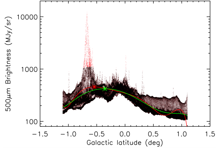
Fig. 2. 500- \mu m brightness values (all the points) as a function of Galactic latitude in the longitude interval 14.5 \leq l \leq 15.5 from the map in Fig. 1b. (This longitude range contains M16, which is clearly visible as the large bump at b \sim -0.7 .) The red thick line is the 7th-order polynomial fit to all points, and the red points are those that are clipped away because they lie above 3 times the rms of the residuals (after subtracting the fit). The green thick line is the 5th-order polynomial fit to all points that survived this clipping (all the black points). The thick crosses indicate the positions of the maxima of each respective fit.
