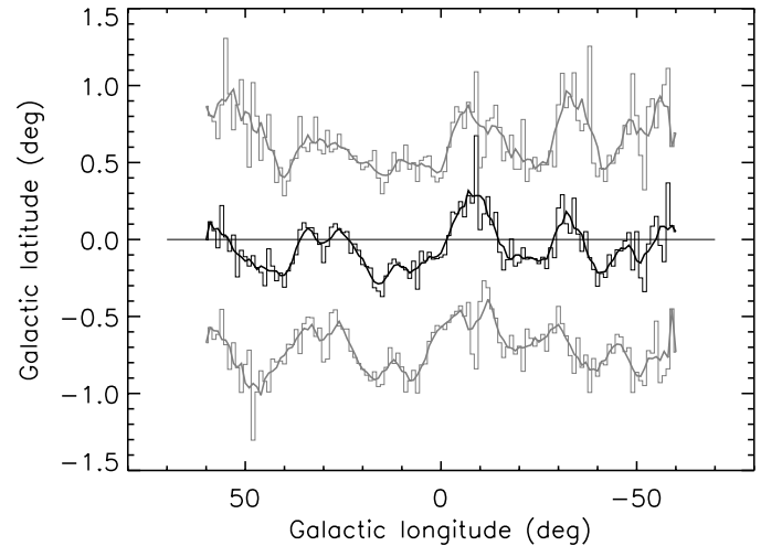
Fig. 3. Distribution in Galactic longitude of the latitude values for the centroid (black histogram) and the upper and lower 50%-level values (grey histograms) of the 500- \mu m emission (see text for a detailed explanation). The thick lines represent the smoothing of the distributions with a 5°-wide running boxcar.
