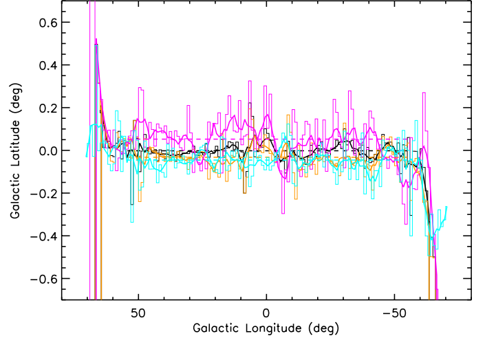
Fig. 9. Same as Fig. 4 for the distribution of MIPS GAL 24\text{ }\mu\text{m} sources alone. The black line is reported straight from Fig. 4 for comparison. The orange line represents the distribution again from the Shenoy et al. (in prep.) catalogue but for sources with fluxes above 3.5 mJy. The cyan line represents the distribution from the WISE 22\text{ }\mu\text{m} source catalogue with flux above 6 mJy. The magenta line instead represents the distribution of the 24\text{ }\mu\text{m} sources from the catalogue in Gutermuth & Heyer (2015) that are above the respective 90% completeness limit.
