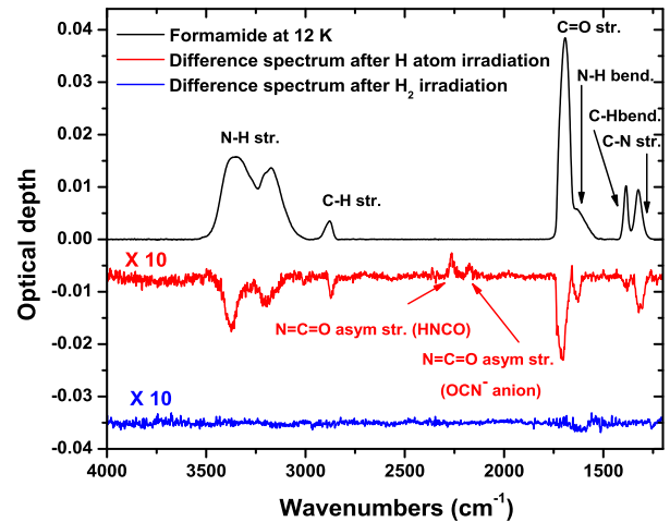
Fig. 1. IR spectrum of a 29 ML thick \text{NH}_2\text{CHO} film at 12 K (black line). The spectrum after irradiation (subtracted from the initial spectrum) of 2 \times 10^{17}\text{ H atoms cm}^{-2} (red line) is reported. The \text{NH}_2\text{CHO} spectrum after irradiation (subtracted from the initial spectrum) of 2.7 \times 10^{17}\text{ H}_2\text{ mol cm}^{-2} (blue line) as obtained in a blank experiment is also shown for comparison purposes. The red and blue curves are offset in ordinate by -0.007 and -0.035 , respectively, for the sake of clarity.
