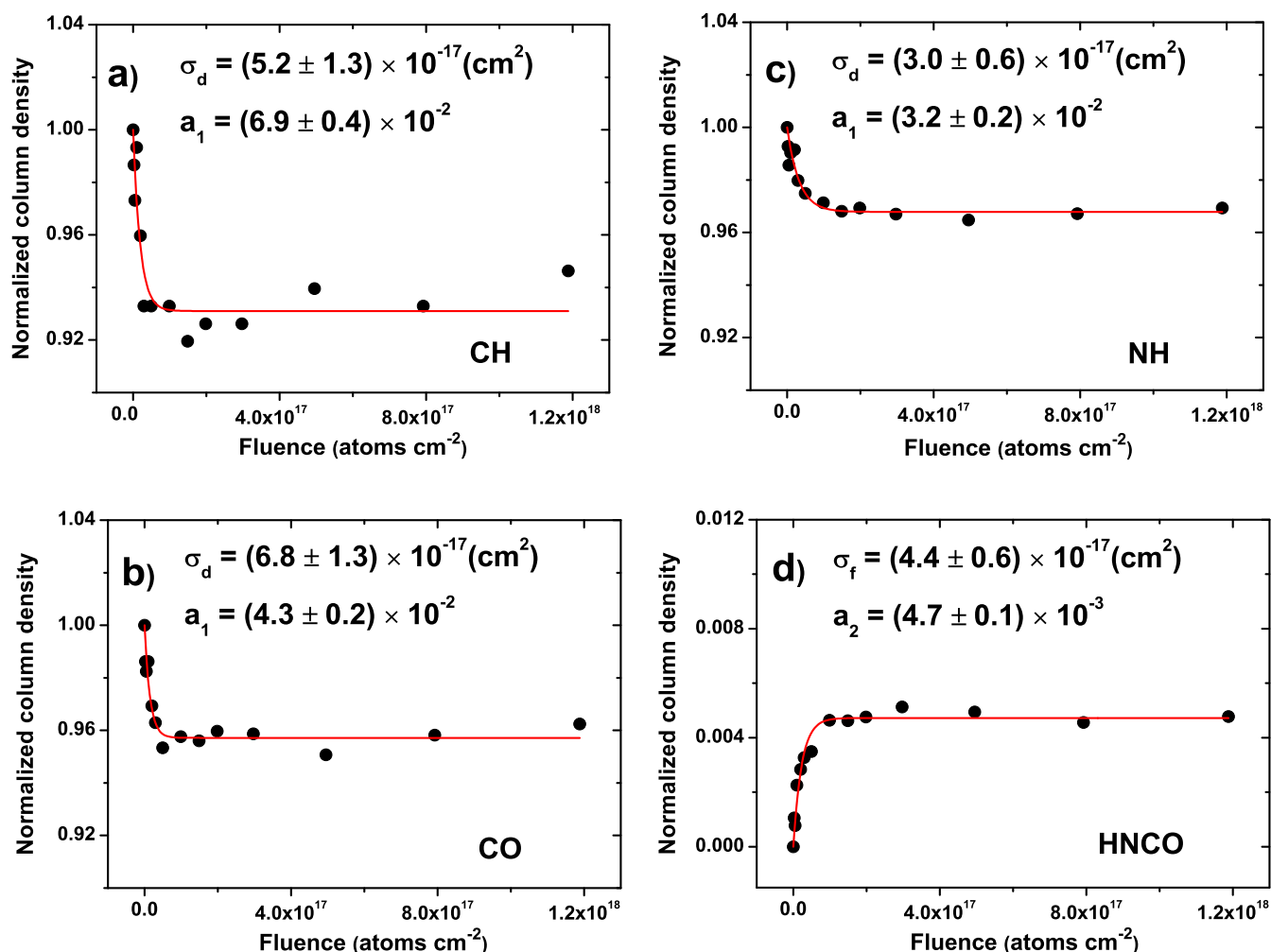
Fig. 2. Evolution with H atom fluence of the C–H (a), C=O (b), N–H (c), and N=C=O (HNCO) (d) normalized column density (filled circles). In the first three cases, the normalization factor is the corresponding initial column densities, while for HNCO, the data are normalized to the initial value of the column density of \text{NH}_2\text{CHO} . The best fit to the data (solid lines), following first order kinetic relations (1 - a_1(1 - e^{-\sigma_d F_H})) and a_2(1 - e^{-\sigma_f F_H}) are also shown. The first equation refers to the destruction with the boundary condition that considers a residual reactant for F_H = \infty (i.e., H atoms cannot react with the deeper ice layers). The second equation refers to the formation limited by the availability of the reactants. The estimated destruction ( \sigma_d ) and formation ( \sigma_f ) cross-sections and the asymptotic destruction of \text{NH}_2\text{CHO} ( a_1 ) and asymptotic formation of HNCO ( a_2 ) are also reported.
