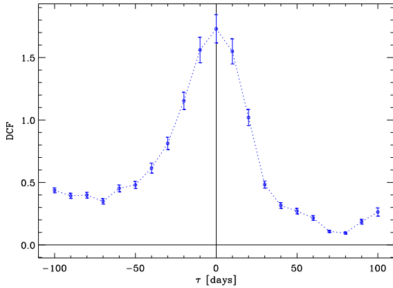
Figure 8. DCF between the \gamma -ray fluxes obtained with five-day time bins and the R -band flux densities with 1 day binning over the whole 2013–2017 period.
