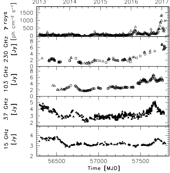
Figure 13. Multifrequency light curve for the period 2013 January 1–2017 February 9 in the following energy bands (from top to bottom): \gamma rays (100 MeV–300 GeV; 5-d time bins, in units of 10^{-8} ph cm ^{-2} s ^{-1} ; Fermi -LAT data), 230 GHz (in units of Jy; triangles: SMA data, squares: IRAM data), 91 and 103 GHz (in units of Jy; ALMA data), 37 GHz (in units of Jy; Metsähovi data), 15 GHz (in units of Jy; OVRO data).
