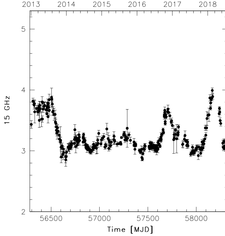
Figure A1. OVRO light curve of CTA 102 at 15 GHz between 2013 January 1 (MJD 56293) and 2018 July 21 (MJD 58320).
