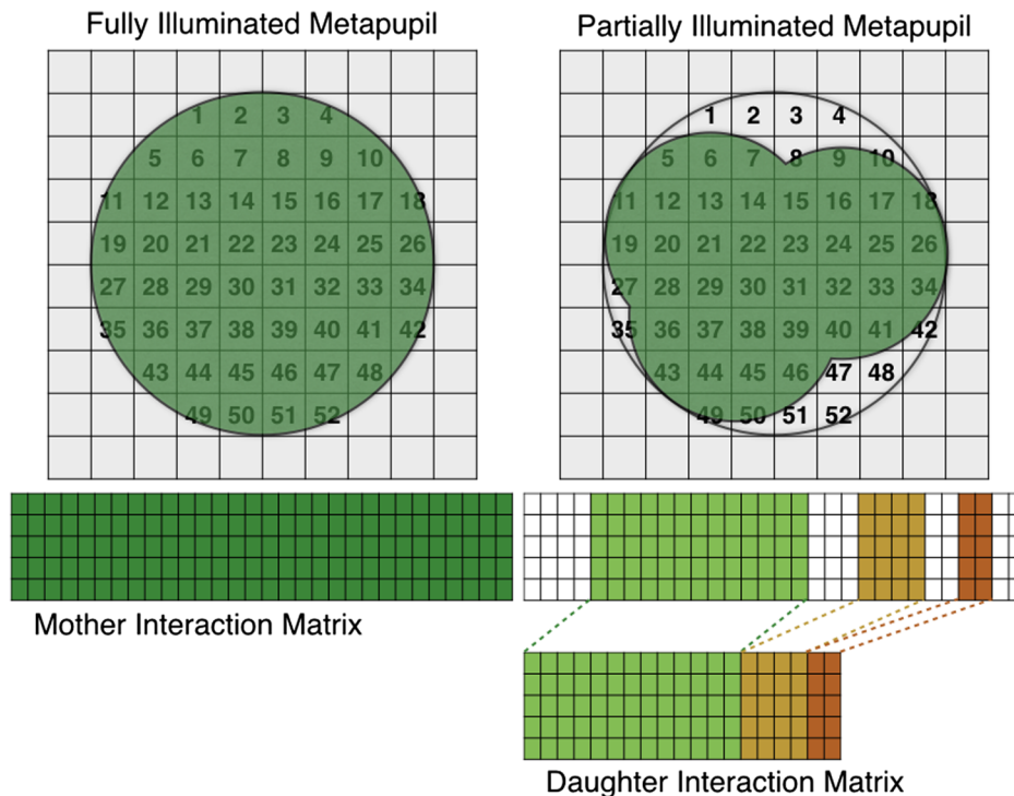
Fig. 8 A schematic diagram explaining the extraction of the daughter-IM from the mother-IM. On the left, the fully illuminated metapupil and the corresponding IM can be seen. On the right, the partially illuminated metapupil appears along with the daughter-IM extracted out of the mother-IM.
