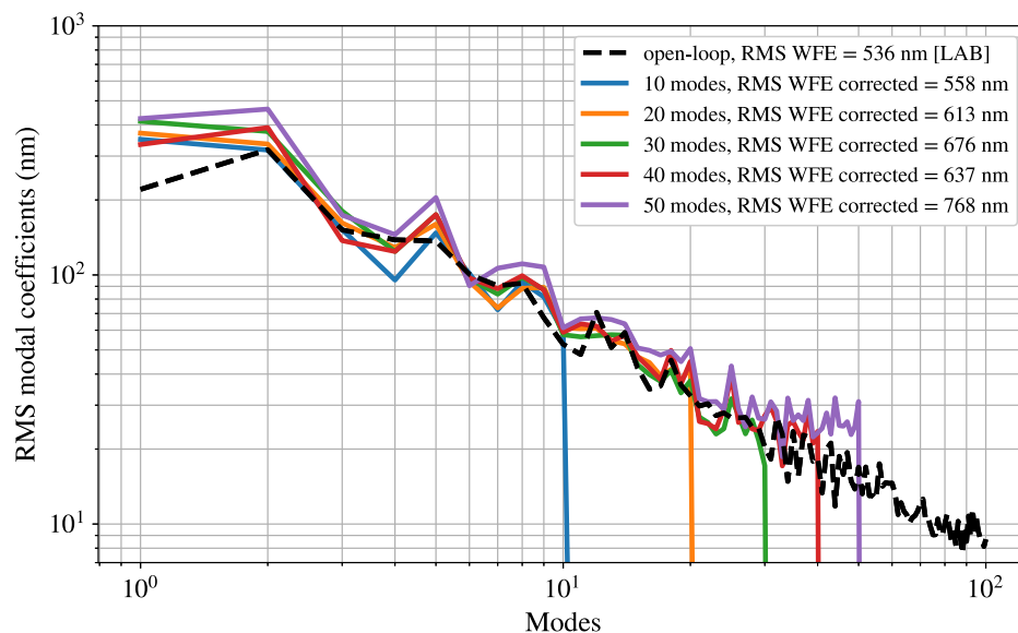
Fig. 13 The RMS value of the modal coefficients versus the modes for the asterism shown in Fig. 12. Although we closed up to 50 modes in the high layer, we noticed instabilities arising for modes higher than 40. Therefore, for the IR image shown in the bottom-right corner of Fig. 12, only the first 40 modes were closed. The RMS WFE are mentioned in the legend.
