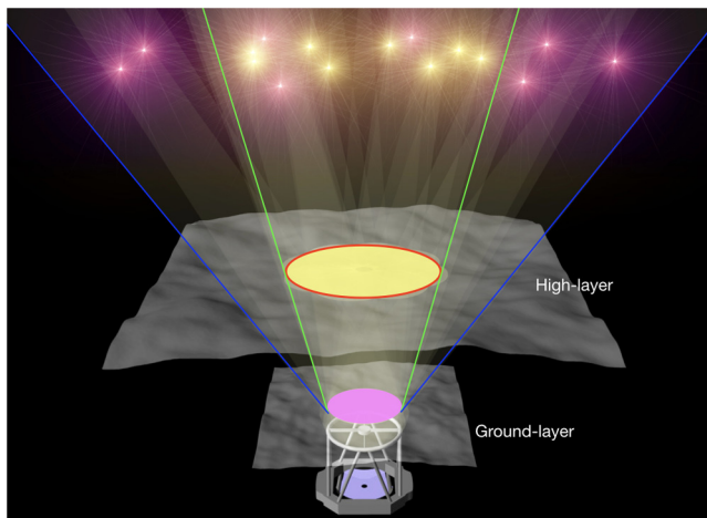
Fig. 1 LN MCAO multiple-FoV approach: The ground layer is sensed using the purple NGs from the 2' to 6' annular FoV and drives the facility ASM of the LBT. The high layer, conjugated to \sim 7100 m away from the telescope pupil along the optical axis, is sensed by the yellow NGs in the inner 2' diameter FoV. A commercial Xintetics DM on the LN bench corrects the aberrations sensed by the HWS. Note that the yellow shaded region within the red circle denotes the metapupil, and the angle subtended by the green lines and blue lines represent the 2' and 6' FoV, respectively.
