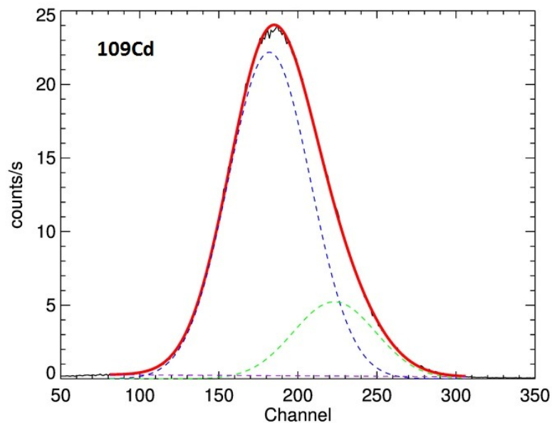
Figure 3: Spectrum of the 22 – 24 keV lines of ^{109}\text{Cd} detected with the GAGG rod ( 3\text{ mm} \times 3\text{ mm} \times 30\text{ mm} ) and the LCT5 SiPM at the nominal overvoltage value of +3 V. The blue dashed line is the gaussian fit of the line at 22 keV, the green dashed line is the gaussian fit of the line at 24 keV, the purple dashed line is the background.
