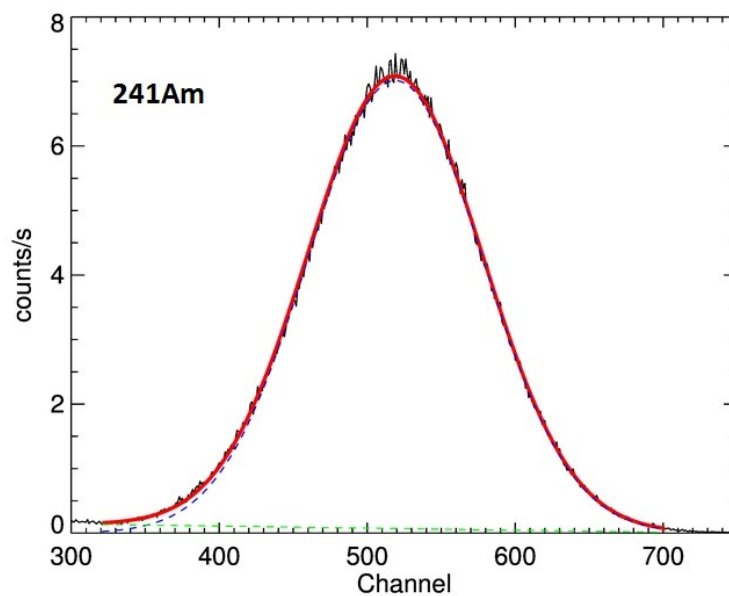
Figure 4: Spectrum of the 59.5 keV line of ^{241}\text{Am} detected with the GAGG rod ( 3\text{ mm} \times 3\text{ mm} \times 30\text{ mm} ) and the LCT5 SiPM at the nominal overvoltage value of +3 V. The blue dashed line is the gaussian fit of the X-ray line, the green dashed line is the background.
