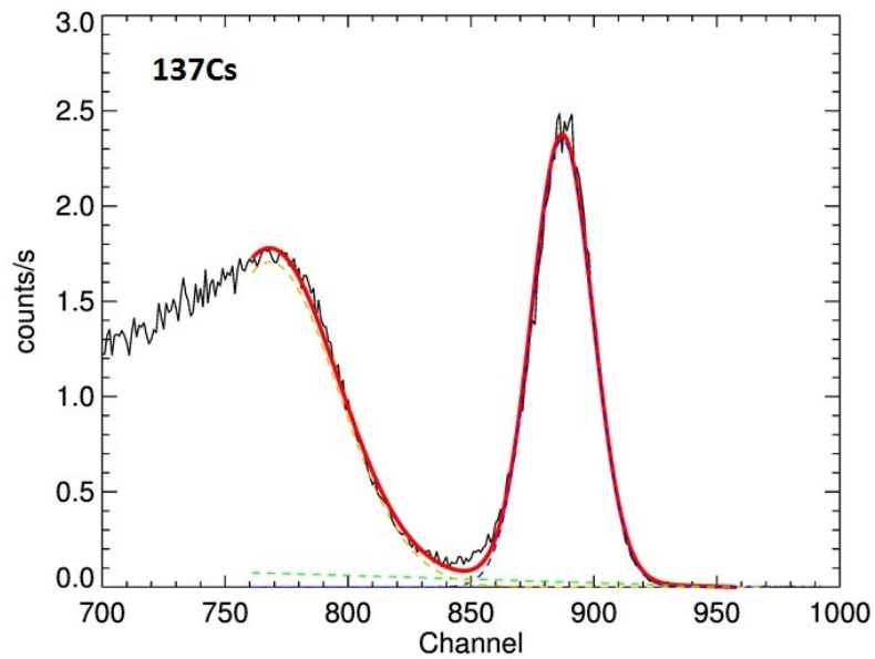
Figure 5: Spectrum of the 662 keV line of ^{137}\text{Cs} detected with the GAGG rod ( 3\text{ mm} \times 3\text{ mm} \times 30\text{ mm} ) and the LCT4 SiPM ( 75\text{ }\mu\text{m} pitch) at the nominal overvoltage value of +3 V. The blue dashed line is the gaussian fit of the X-ray line, the green dashed line is the background and the orange dashed line is the empirical fit of the Compton edge (modelled as the product of a Gauss error function and an exponential function, following the guidelines 12 ).
