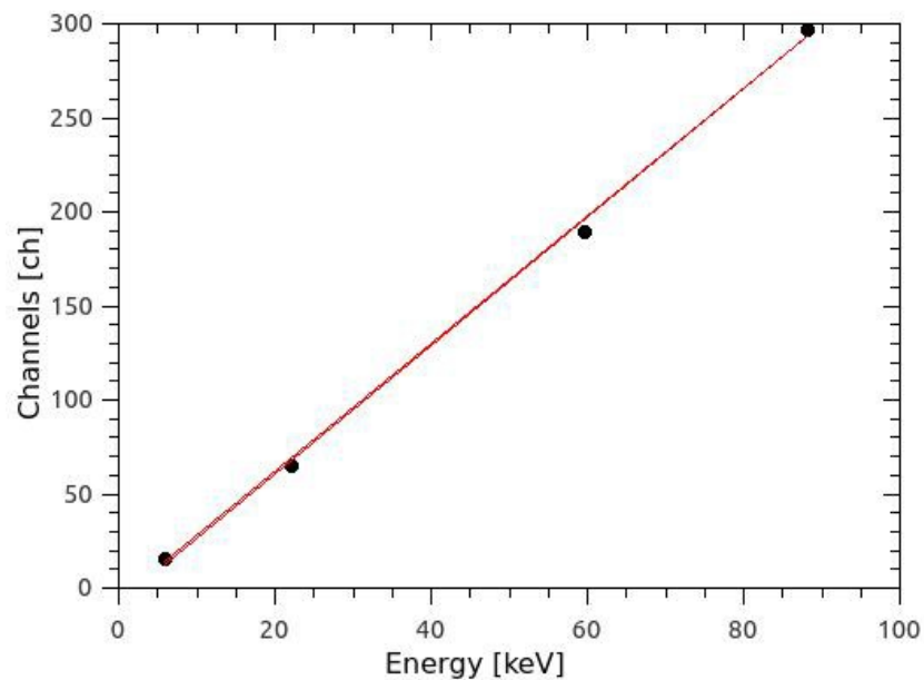
Figure 6: Linearity of the system of GAGG rod ( 3\text{ mm} \times 3\text{ mm} \times 30\text{ mm} ) and LCT5 SiPM (nominal overvoltage of +3 V).
