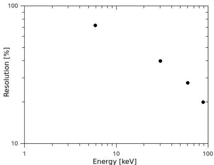
Figure 7: Energy resolution of the system of GAGG rod ( 3\text{ mm} \times 3\text{ mm} \times 30\text{ mm} ) and LCT5 SiPM as a function of the energy. The energy resolution is defined as the ratio between the FWHM and the peak position.
