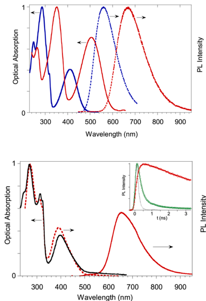
Fig. 2. Top: Normalized optical absorption (solid lines) and PL (dashed lines) spectra of chromophores 1 (blue lines) and 2 (red lines) in 10^{-4} M dichloromethane (DCM) solutions. Bottom: Normalized optical absorption (black solid line), PLE (red dotted line, \lambda_{em} = 655 nm) and PL (red solid line, \lambda_{ex} = 400 nm) spectra of 1:2 film. In the inset the PL time decay of 1:2 film ( \lambda_{em} = 533 nm, green diamonds; \lambda_{em} = 650 nm, red diamonds), fits (solid lines, ESI) and prompt (grey dotted line). \lambda_{ex} = 408 nm.
