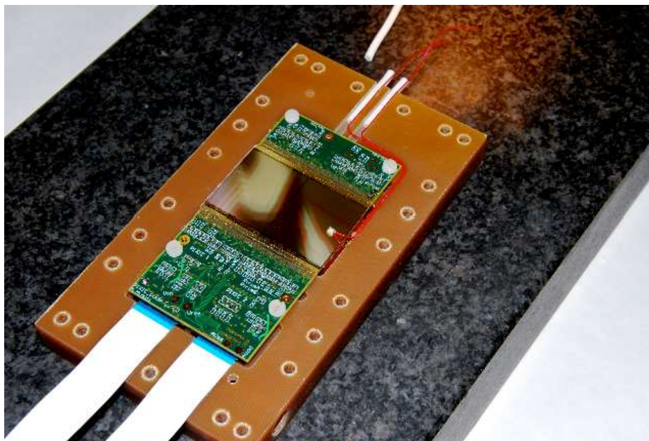
Figure 4-27: A 2×1 linear hybrid module mounted onto the motherboard PCB.
