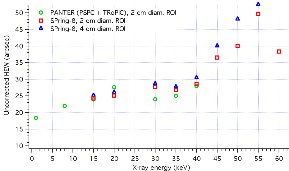
Figure 3-19: the HEW of the MS297R9, measured at PANTER and SPring-8. For the SPring-8 measurements, two ROIs were considered. The HEW, as expected, exhibits an increasing trend with the X-ray energy.
