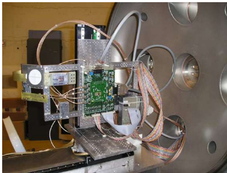
Figure 4-18 The Motherboard and the Carrier PCBs inside the vacuum tank. On the right are visible the connectors fixed on the door tank.
