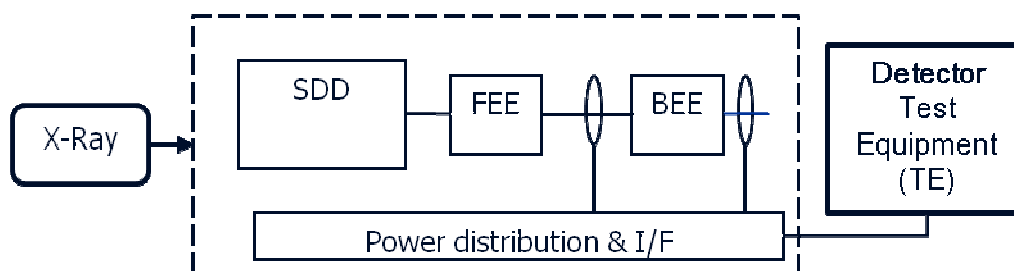
Figure 6-5: Test Configuration for AIT and Calibration at Detector Level
