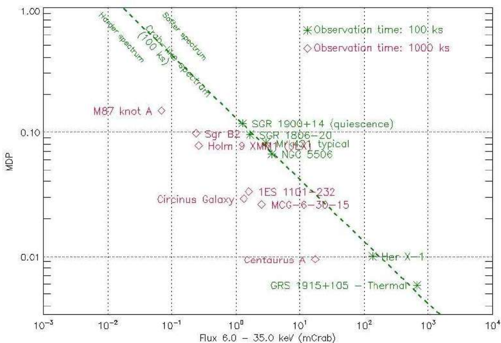
Figure 5-12: Minimum Detectable polarization for the MEP
