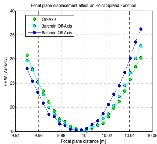
Figure 3-3: degradation of the angular resolution HEW due to the displacement of the detector from the best focal plane. (left) 1 keV and (right) 30 keV.
