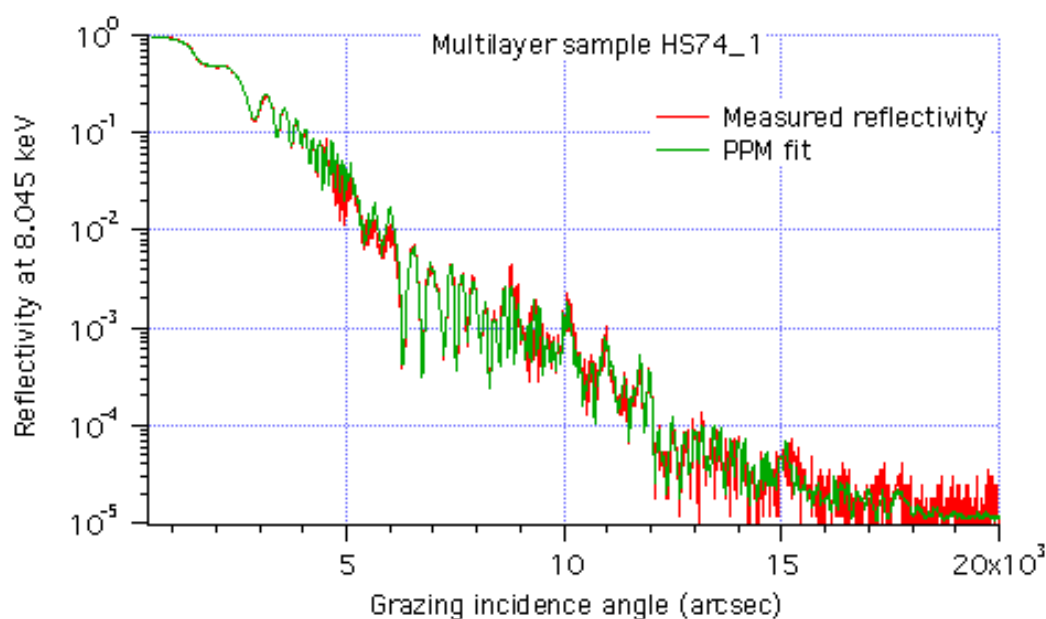
Figure 3-10: the measured reflectivity (red) of a Pt/C graded multilayer sample deposited for this project. In green we also plot the inferred reflectivity model, assuming a 4.5 Å of roughness rms.
