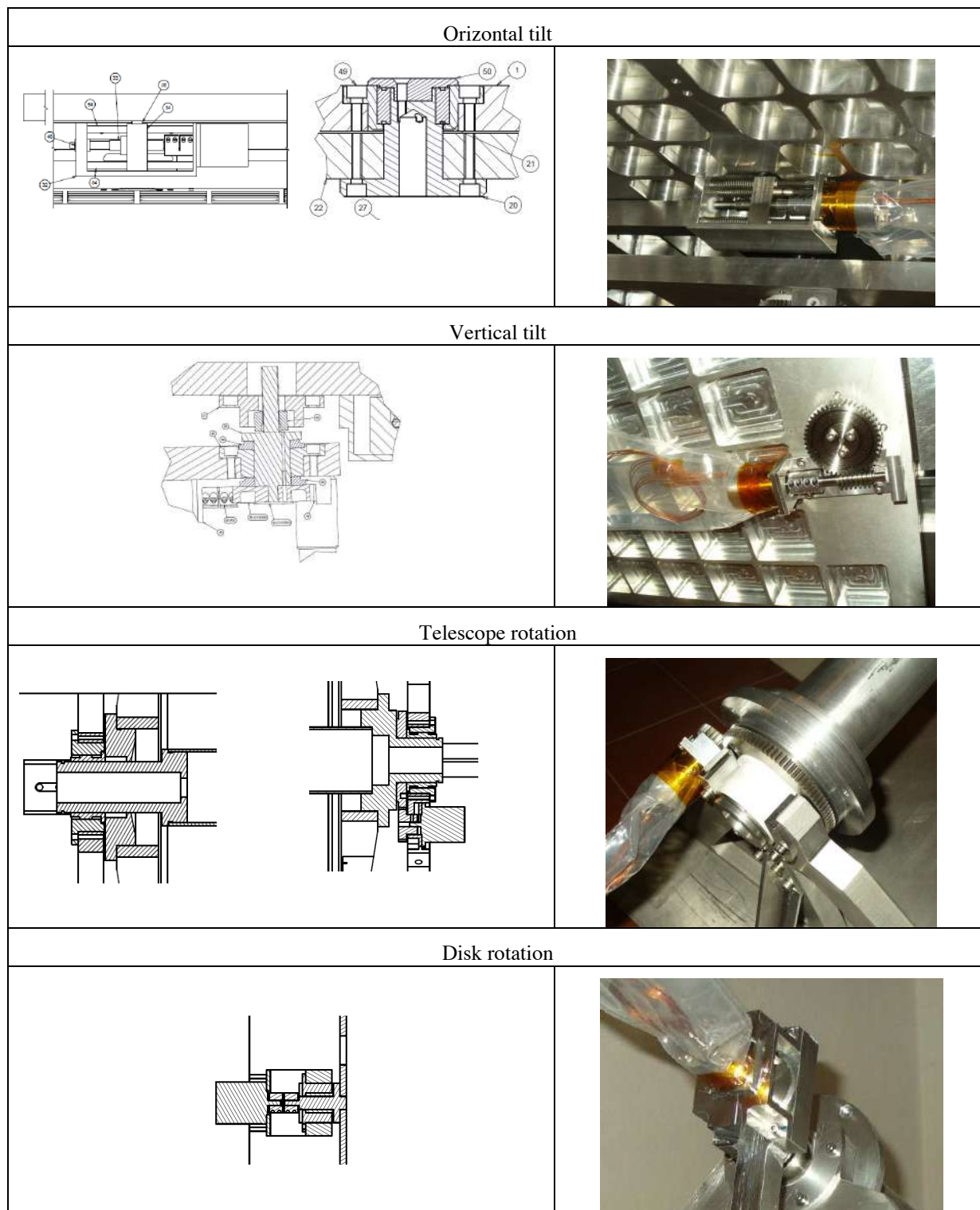
Figure 6-15: jig details
