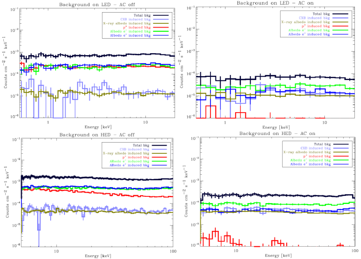
Figure 4-45: Simulated background spectra, in \text{counts cm}^{-2} \text{s}^{-1} \text{keV}^{-1} , for the Case B configuration. Top panels: LED background, in the 0.5 – 20 keV energy range, in “AC off” (left) and “AC on” (right) mode; bottom panels: HED background, in the 5 – 100 keV energy range, in “AC off” (left) and “AC on” (right) mode.
