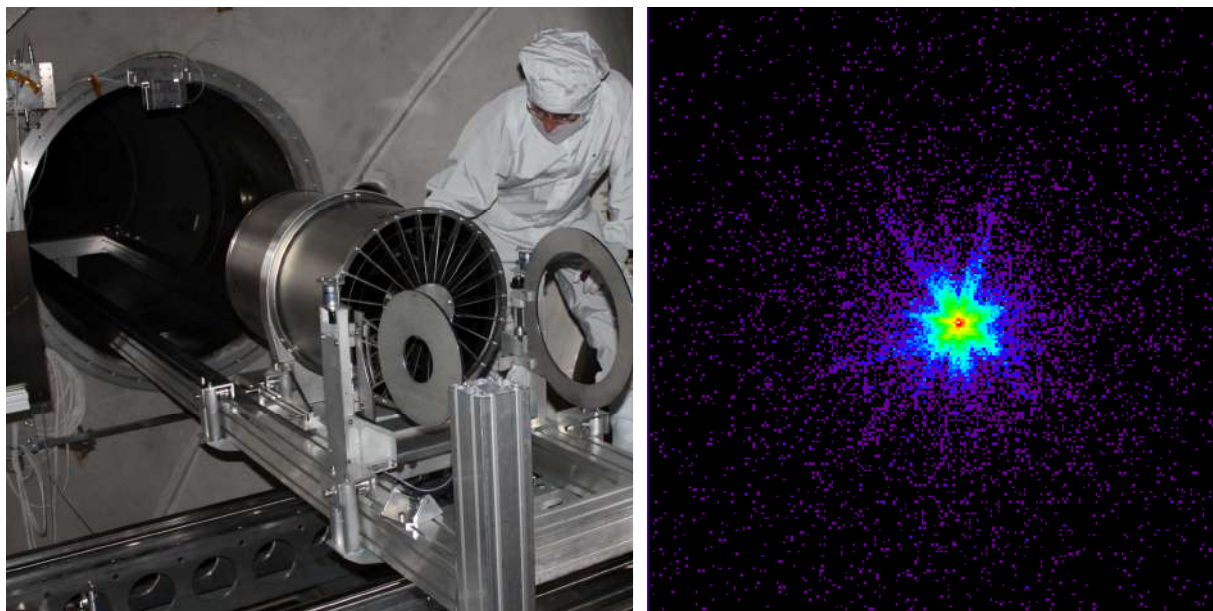
Figure 3-14: a mirror module prototype, including a W/Si multilayer-coated mirror shell, tested at PANTER. The focal spot seen in the TRoPIC CCD detector in a X-ray energy band of 20-35 keV. The HEW is 22 arcsec, very close to the specification ( < 20 arcsec for E < 30 keV).
