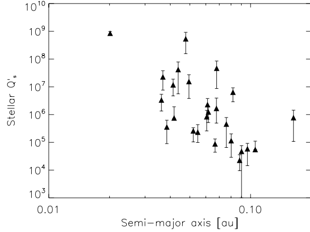
Figure 6: Lower limits of the modified tidal quality factor Q'_s of stars hosting eccentric planets computed by using Eq. (9) in Matsumura et al. (2008). The large error bars are mainly due to the uncertainties on system ages.
