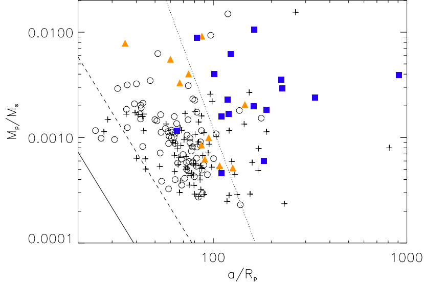
Figure 2: Updated tidal diagram of the 211 transiting giant planets considered in this study. Empty circles show the position of giant planets with well-determined circular orbits, that is with eccentricities consistent with zero and 1\sigma uncertainty \sigma_e < 0.05 ; crosses indicate likely circular orbits but with large uncertainties \sigma_e > 0.05 ; orange triangles display significant but small eccentricities, i.e. e \leq 0.1 ; and blue squares e > 0.1 . Solid and dashed lines show the position of a planet with R_p = 1.2 R_{Jup} and semi-major axis a = a_R and a = 2a_R . The dotted line displays the 1-Gyr circularisation time scale for P = 3 d, Q'_p = 10^6 , and e = 0 .
