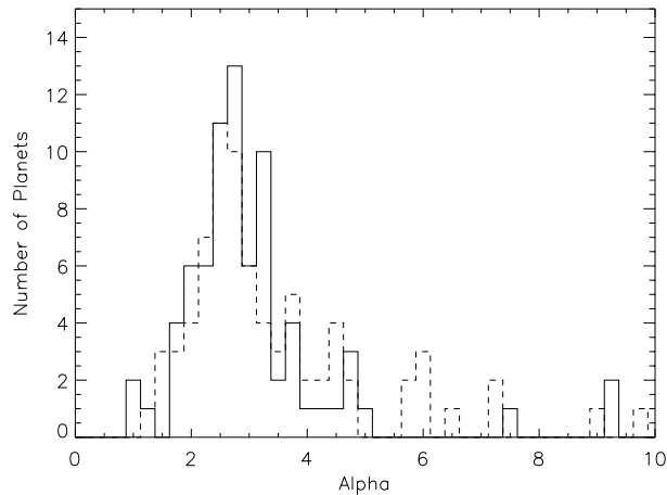
Figure 3: Distribution of \alpha = a/a_R for well-determined circular orbits ( \sigma_e < 0.05 , solid line) and likely circular orbits (eccentricities consistent with zero but with large errors \sigma_e > 0.05 , dashed line). Both distributions are not corrected for the transit probability.
