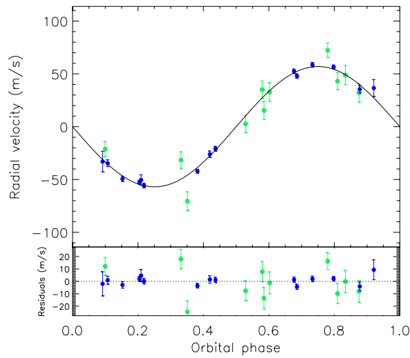
Figure 1: HARPS-N (blue circles) and SOPHIE (green circles) RV measurements of WASP-13. Note the high-accuracy and precision radial velocities collected with HARPS-N with respect to the literature data.
