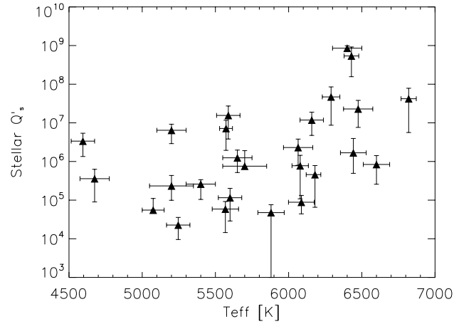
Figure 7: Lower limits of the modified tidal quality factor Q'_s of stars hosting eccentric planets as a function of stellar effective temperature.
