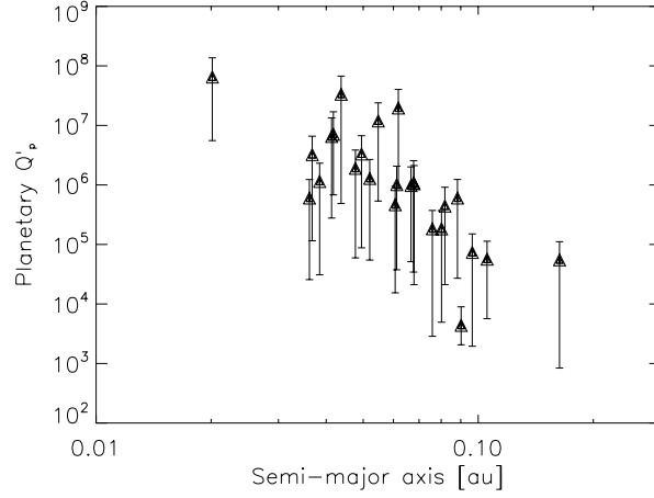
Figure 5: Lower limits of the planetary modified tidal quality factor Q'_p for eccentric orbits computed by using Eq. (8) in Matsumura et al. (2008). The large error bars are mainly due to the uncertainties on system ages.
