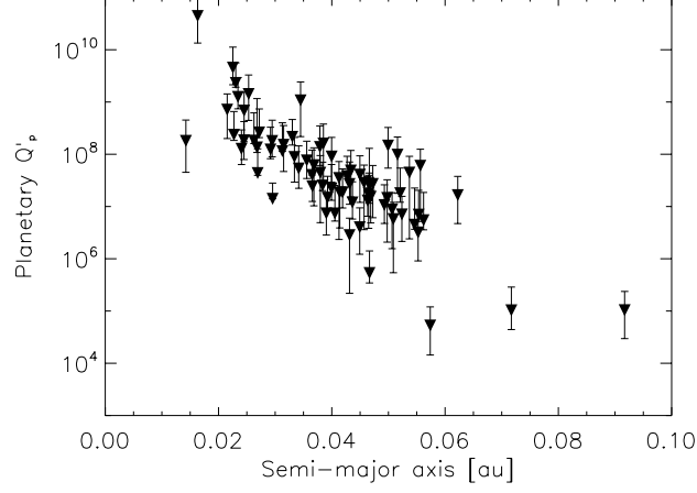
Figure 4: Upper limits of the planetary modified tidal quality factor Q'_p for clearly circular orbits ( \sigma_e < 0.05 ) computed by using Eq. (7) in Matsumura et al. (2008). The large error bars are mainly due to the uncertainties on system ages.
