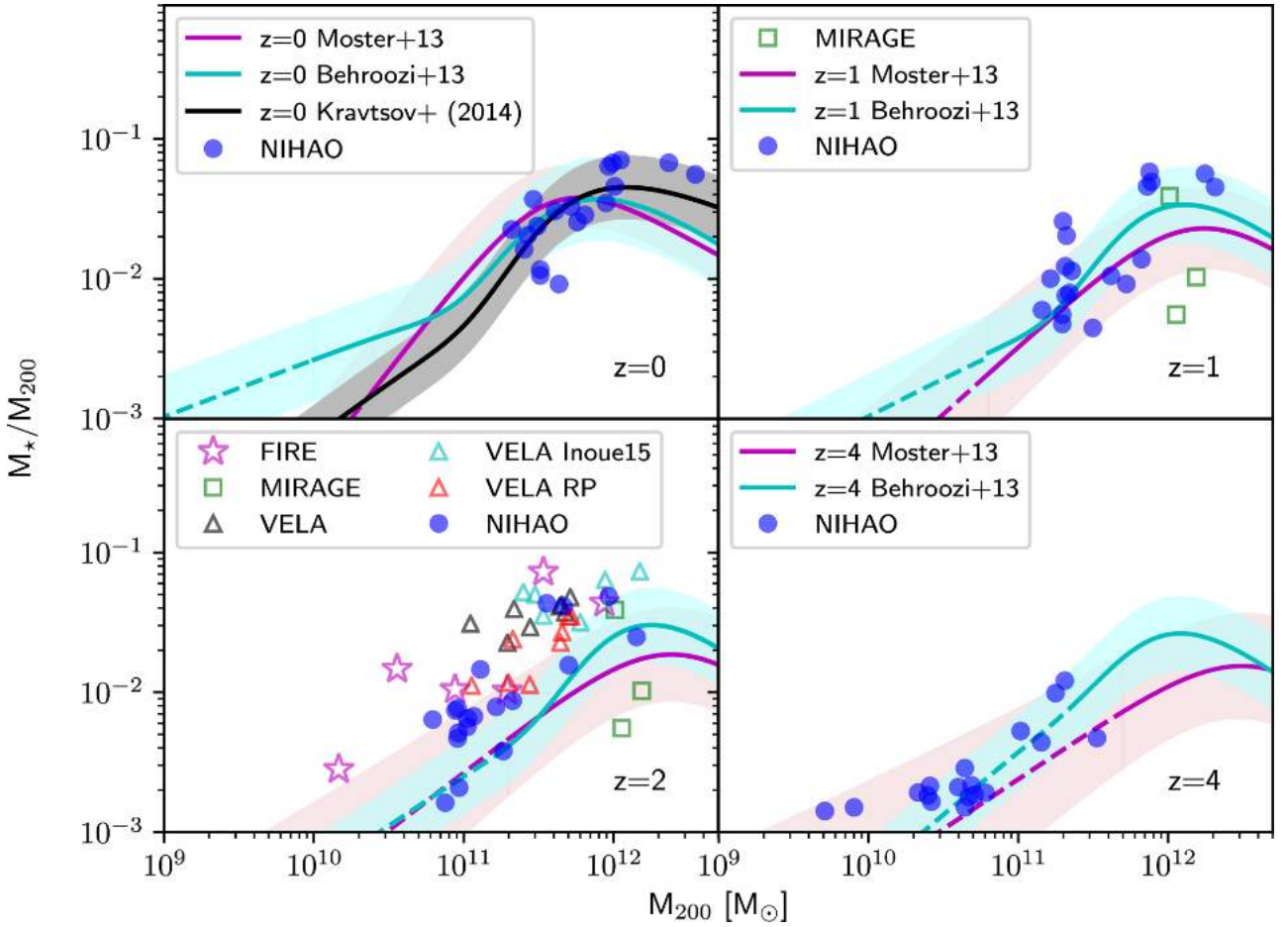
Figure 1. Evolution of the stellar mass versus halo mass relation for the selection of hosts. Redshift z = 0 (top left-hand panel), 1 (top right-hand panel), 2 (bottom left-hand panel) and 4 (bottom right-hand panel). For all redshifts shown, the simulations agree well with constraints from halo abundance matching (Behroozi, Wechsler & Conroy 2013; Moster, Naab & White 2013; Kravtsov, Vikhlinin & Meshcheryakov 2014). Where the relations are extrapolated into mass scales without observational constraints, the lines are shown in dashed line style.
